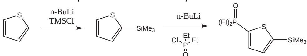
Scheme 1-34: Phosphonate introduction on thiophene
