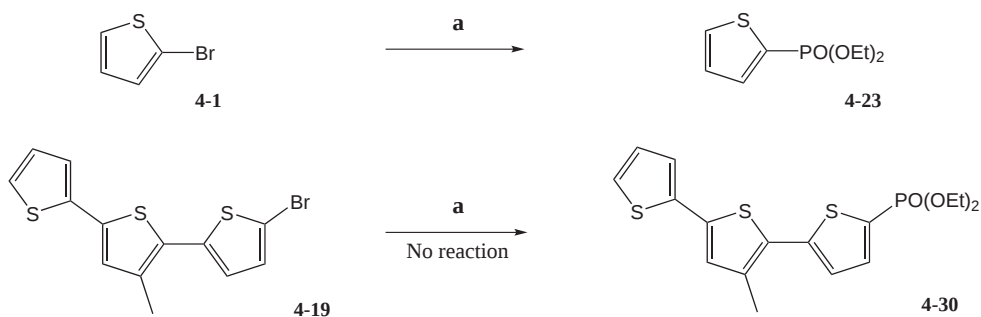
Scheme 4-13: Fosfonation reactions
