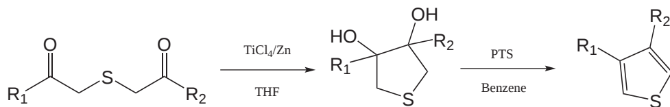
Scheme 1-26: formation of thiophene oligomers from 3-thiapentanes-1,5-diones 69
