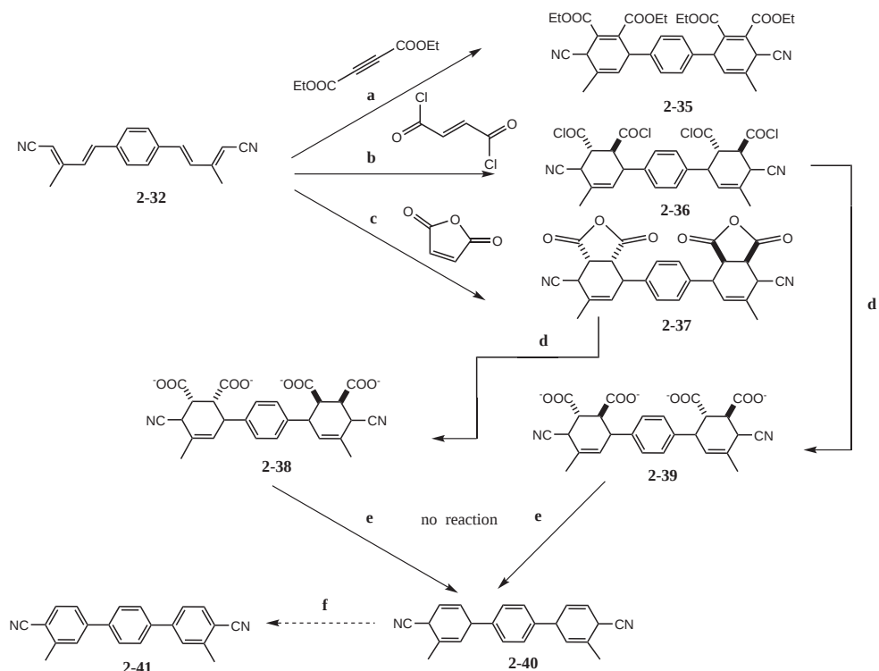
Scheme 2-9:
