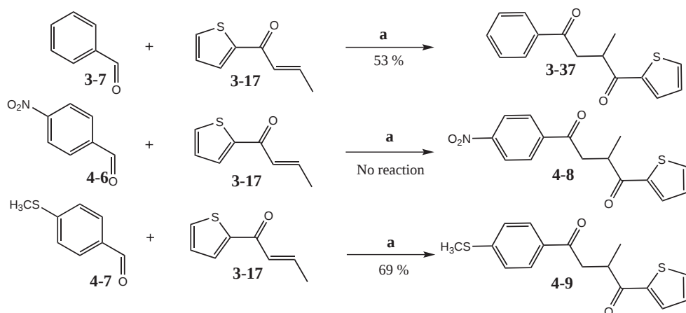
Scheme 4-6: Stetter reactions starting with benzaldehydes
