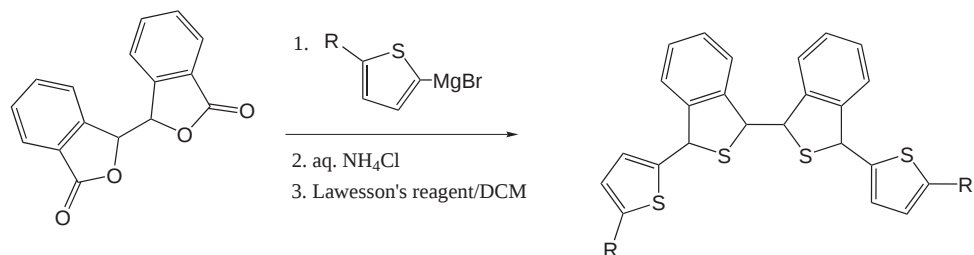
Scheme 1-26: formation of thiophene oligomers from 3-thiapentanes-1,5-diones 69
