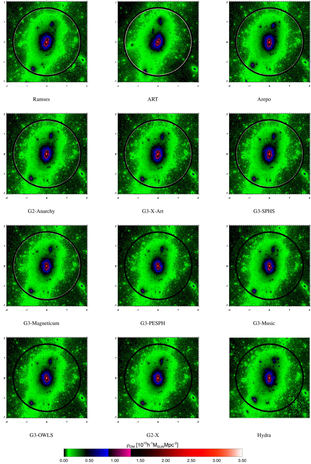
Figure A2. Projected density of the dark matter halo in the non-radiative simulations at z = 0 for each method as indicated. The box is 2 h^{-1} \text{Mpc} on a side. The white circle indicates M_{\text{crit}}^{200} for the halo, the black circle the same but for the G3-MUSIC simulation.
