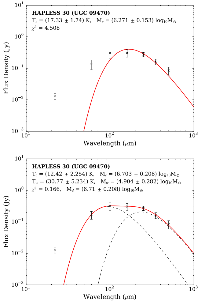
Figure 5. Example dust SED of UGC 09470 (HAPLESS 30), with one- and two-temperature component MBB fits attempted (upper and lower panels, respectively). Both used a fixed \beta = 2 . Grey points represent upper limits in the fitting routine. This is an example of a galaxy for which a one-component dust model systematically underestimates the flux at both 100 and 500 \mu\text{m} , whilst overestimating it at 160 \mu\text{m} .
