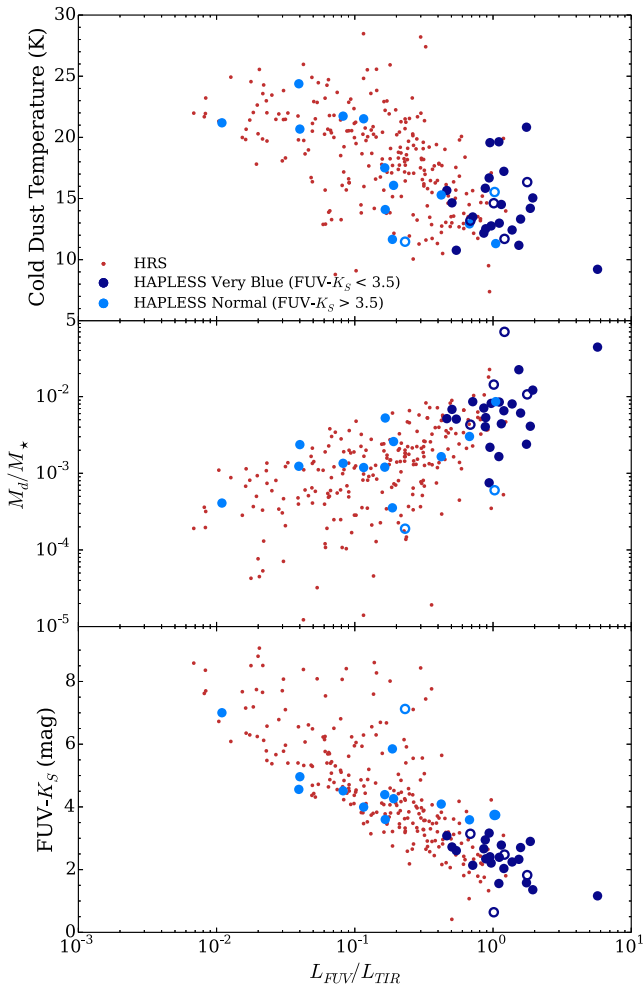
Figure 15. Scaling relations with L_{\text{FUV}}/L_{\text{TIR}} for the HAPLESS and HRS. Upper: cold dust temperature against L_{\text{FUV}}/L_{\text{TIR}} . Centre: M_d/M_* against L_{\text{FUV}}/L_{\text{TIR}} ; counter-intuitively, the more dust-rich a galaxy, the larger the proportion of FUV photons that go unabsorbed. Lower: FUV- K_S colour against L_{\text{FUV}}/L_{\text{TIR}} ; correlation is very tight for bluer galaxies, but far weaker for redder galaxies.
