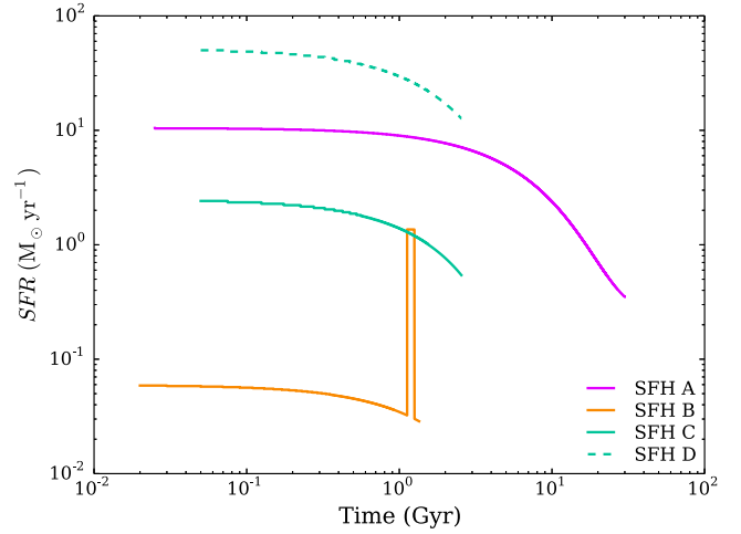
Figure B1. The SFHs used to model the HAPLESS galaxies. SFH A follows the evolution of the MW (pink, uppermost solid track; Yin et al. 2009) with initial gas mass M_g(0) = 4 \times 10^{10} M_\odot and initial SFR \psi(0) = 10 M_\odot \text{ yr}^{-1} . SFH B (orange, lowermost solid track) has initial gas mass M_g(0) \sim 3 \times 10^9 M_\odot and initial SFR 0.058 M_\odot \text{ yr}^{-1} with a burst at 1 Gyr superimposed on top of the exponentially declining rate. SFH C (orange, middle solid track) has M_g(0) = 5.5 \times 10^9 M_\odot and initial SFR 2.4 M_\odot \text{ yr}^{-1} and exponentially declines until reaching a gas fraction of f_g \sim 0.6 at 2.5 Gyr. SFH D (turquoise, dashed track) is a scaled version of SFH C ( \times 20 ).
