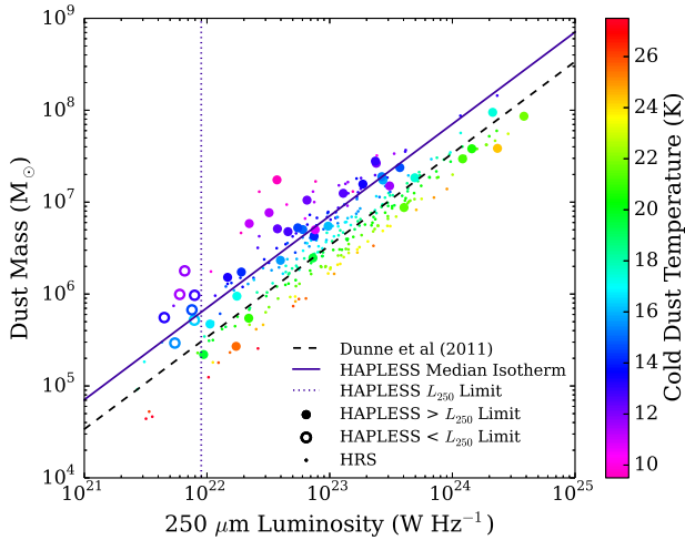
Figure 11. Dust mass against 250 \mu\text{m} luminosity for the HAPLESS and the HRS, colour-coded by cold dust temperature. Also shown are the median dust temperature (solid) for the HAPLESS sources and the relationship in Dunne et al. (2011, dashed). Filled circles show the HAPLESS luminosity complete sub-sample.
