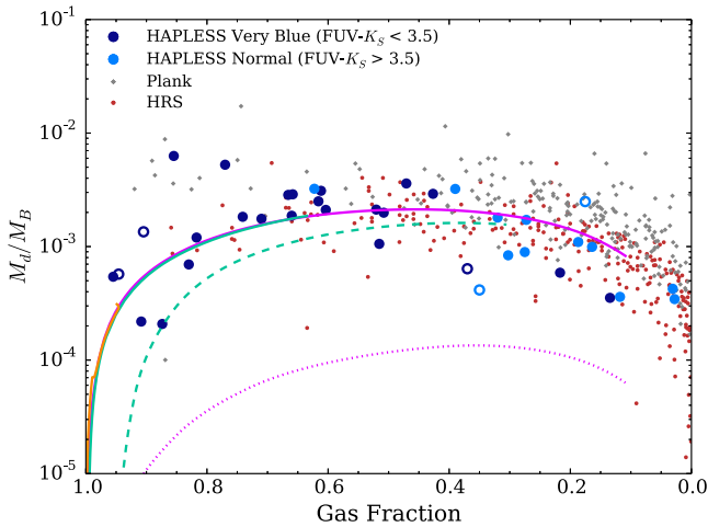
Figure 21. M_d/M_B against gas fraction for the three samples. Note that the x-axis of this plot goes from a gas fraction of 1 to 0. The curves show the results from the chemical evolution model for different SFHs (Appendix B1, Table 8) including SFH A – consistent with the Milky Way (purple; Yin et al. 2009); SFH B – exponentially declining SFR with initial value of 0.06 M_{\odot} \text{ yr}^{-1} and a burst (orange); SFH C – an exponentially declining rate, but with higher initial SFR of 2.4 M_{\odot} \text{ yr}^{-1} (tourquoise); and finally SFH D – a scaled version of SFH C ( \times 20 , tourquoise dashed). The dotted purple line is SFH A (MW) with dust from LIMS only.
