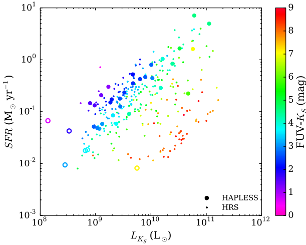
Figure 17. The relationship between L_{K_S} and SFR , colour-coded by FUV– K_S colour (indicating morphology), for the HAPLESS and the HRS galaxies. Hollow circles show galaxies beneath the luminosity limit of the sample.
