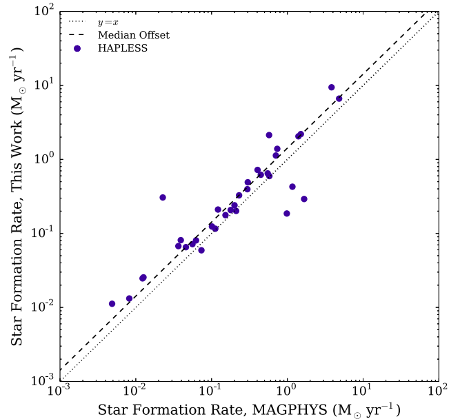
Figure 7. The SFRs calculated using equation (7) compared to those derived by De Vis et al. (in preparation) by fitting the full UV-submm SEDs of our sample using MAGPHYS da Cunha et al. (2008). The offset between the two prescriptions is by a factor of 1.42, as indicated by the dashed line.
