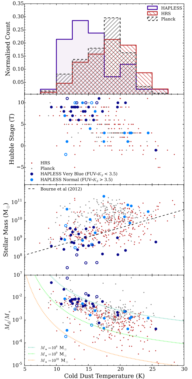
Figure 13. Cold dust temperatures relations for the HAPLESS, HRS, and Planck C13N13 galaxies. From top to bottom – 1st: the distribution of cold dust temperatures. 2nd: the relation between morphological type and cold dust temperature; HAPLESS is heavily skewed towards cold late-type galaxies. 3rd: stellar mass versus cold dust temperature with the relation from Bourne et al. (2012). 4th: M_d/M_* against cold dust temperature. Curves represent different observing limits in M_d/M_* due to the cold dust temperature for a given value of M_* . Hollow circles indicate galaxies that are beneath the luminosity-limit of the sample.
