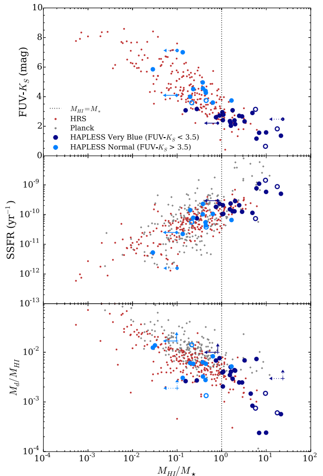
Figure 19. Trends with M_{\text{HI}}/M_\star (i.e. gas richness) for the HAPLESS, HRS, and Planck C13N13 samples. Upper: FUV– K_S versus M_{\text{HI}}/M_\star . Blue colours are strongly associated with higher gas-to-stellar mass fractions; The (FUV– K_S < 3.5 ) colour criterion we use to define the curious very blue galaxies transpires to correspond to M_{\text{HI}} \approx M_\star (vertical dotted line). Centre: M_{\text{HI}}/M_\star against SSFR. Lower: M_d/M_{\text{HI}} against M_{\text{HI}}/M_\star . Hollow circles indicate galaxies that are beneath the luminosity-limit of the sample. HIPASS 3 \sigma upper limits (equation 5) are shown (dotted in the case of galaxies not in our 250 \mu\text{m} luminosity-limit sub-sample.)
