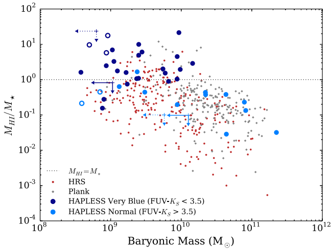
Figure 20. M_{\text{HI}}/M_* against the baryonic mass of the HAPLESS, HRS, and Planck C13N13 samples. The dotted line indicates M_{\text{HI}}/M_* = 1 . Symbols as in Fig. 19.
