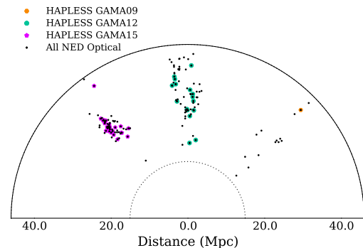
Figure 2. Polar plot of the volume sampled by HAPLESS in the GAMA09, GAMA12, and GAMA15 fields (right to left). The positions of the HAPLESS galaxies are shown (same symbols as Fig. 1). Also shown are all the optical sources with redshifts that place them in the volume. The inner distance limit of D = 15 Mpc is demarked by the dotted black line.
