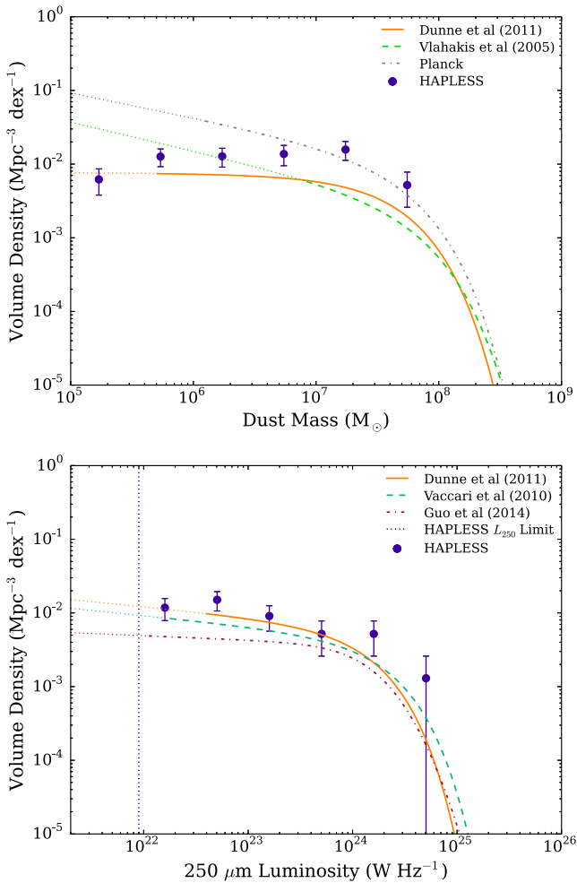
Figure 10. Upper: the HAPLESS DMF (with appropriate incompleteness corrections applied) compared with those of Planck C13N13, Vlahakis et al. (2005), and the H-ATLAS SDP functions from Dunne et al. (2011). Lower: the 250 \mu\text{m} luminosity function of HAPLESS compared with the z < 0.1 H-ATLAS samples from Dunne et al. (2011), Guo et al. (2014) and the z < 0.2 sample from HerMES (Vaccari et al. 2010). The error bars on points represent Poisson uncertainty. The functions are plotted as dotted lines in the regions where they are extrapolated. All have been adjusted to our \kappa_d and cosmology.
