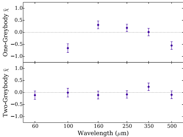
Figure 6. The mean residual across the sample between the model and the data as a fraction of the uncertainty, \bar{\chi} , in each band, for the one- and two-temperature MBB fits (example in Fig. 5). The single MBB approach systematically overestimates the flux at 160 \mu\text{m} whilst underestimating it at 100 and 500 \mu\text{m} . The error bars show the uncertainty on the data points, defined by \sigma = N^{-1/2} .
