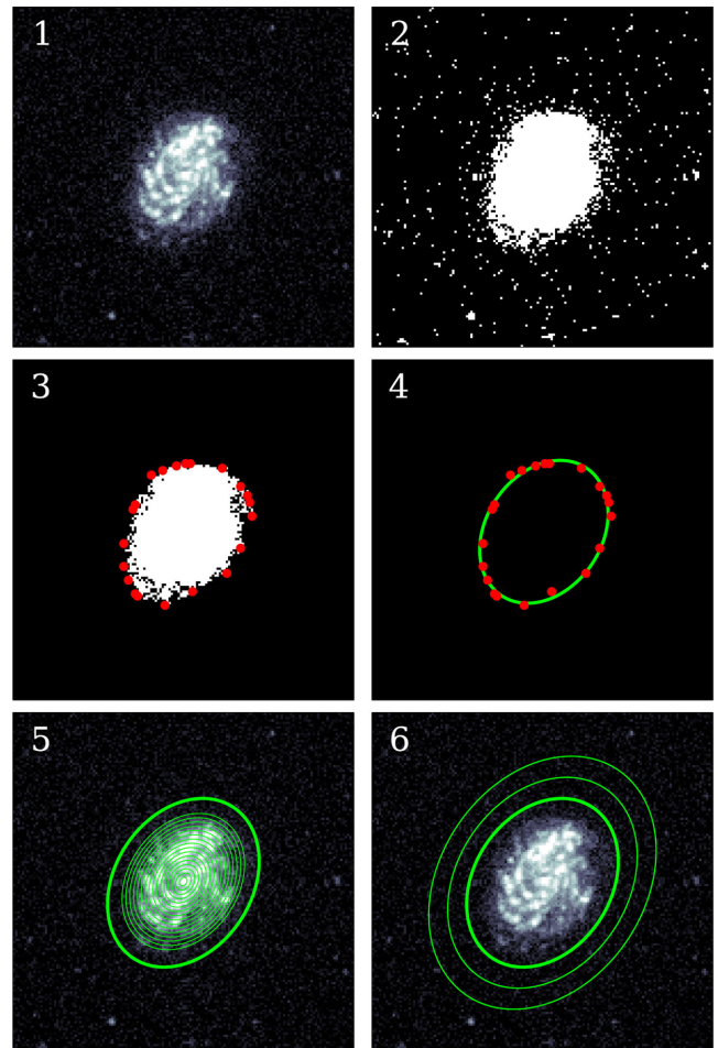
Figure 4. Illustration of the stages of our aperture-fitting process, using GALEX FUV imagery of galaxy NGC 5584 (HAPLESS 14) as an example. Panel 1 shows the inner 500 arcsec \times 500 arcsec portion of the cutout centred upon the target source. Panel 2 shows all of the pixels in the cutout with SNR > 3 . Panel 3 shows the significant pixels of the target source, contained within their convex hull (red points). Panel 4 shows an ellipse fitted to the convex hull; this ellipse provides the position angle and axial ratio of the source aperture. Panel 5 depicts the incremental annuli used to establish the semimajor axis at which annular flux falls to SNR < 2 (thin concentric lines); 1.2 times this distance is then used as the semimajor axis of the source aperture (thick line). Panel 6 demonstrates the final source aperture (thick line) and sky annulus (thin lines). The apertures at all bands for a given source are then compared to select the largest, which is then employed for all bands.
