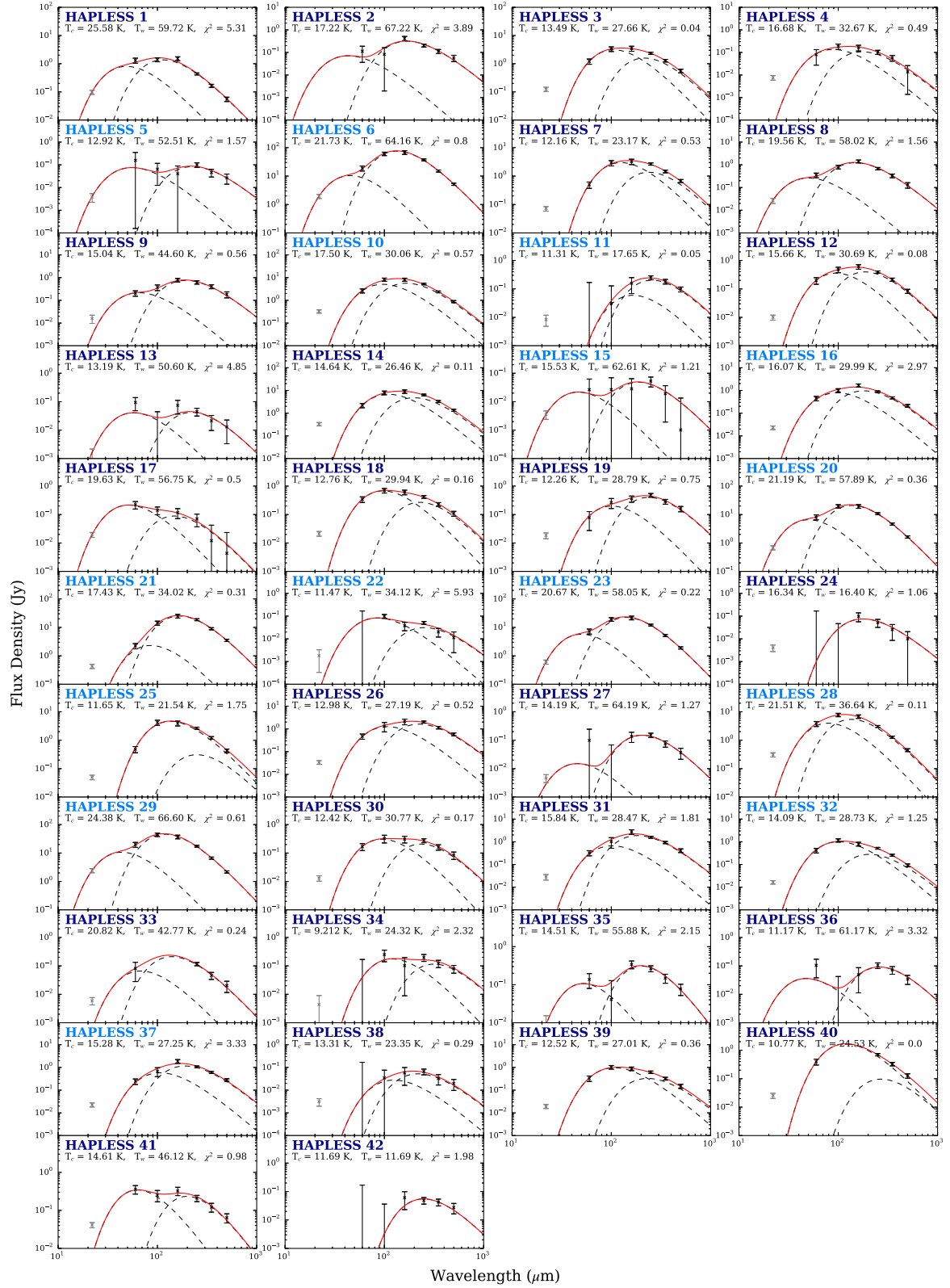
Figure A2. SEDs for the HAPLESS sample. The two-temperature MBB fits are shown in red, with the contributions from the warm and cold dust components shown by the dashed curves. The grey 22 \mu\text{m} point was treated as an upper limit. Sources with dark blue names satisfied the \text{FUV}-K_S < 3.5 colour criterion necessary to be counted amongst the curious blue sub-population; sources with light blue names did not.
