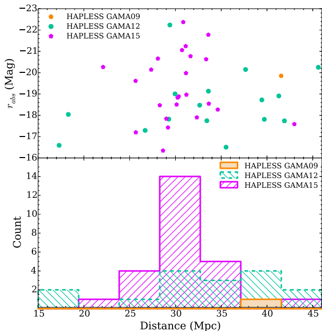
Figure 1. Upper: absolute r -band magnitude against distance, for the 42 galaxies of the HAPLESS sample. The different colours and shapes denote whether the galaxy lies in the GAMA09 (orange hexagons), GAMA12 (green circles), or GAMA15 (purple pentagons) fields sampled as part of the H -ATLAS Phase 1 data release. Lower: the distance distribution of HAPLESS sources in the different fields.
