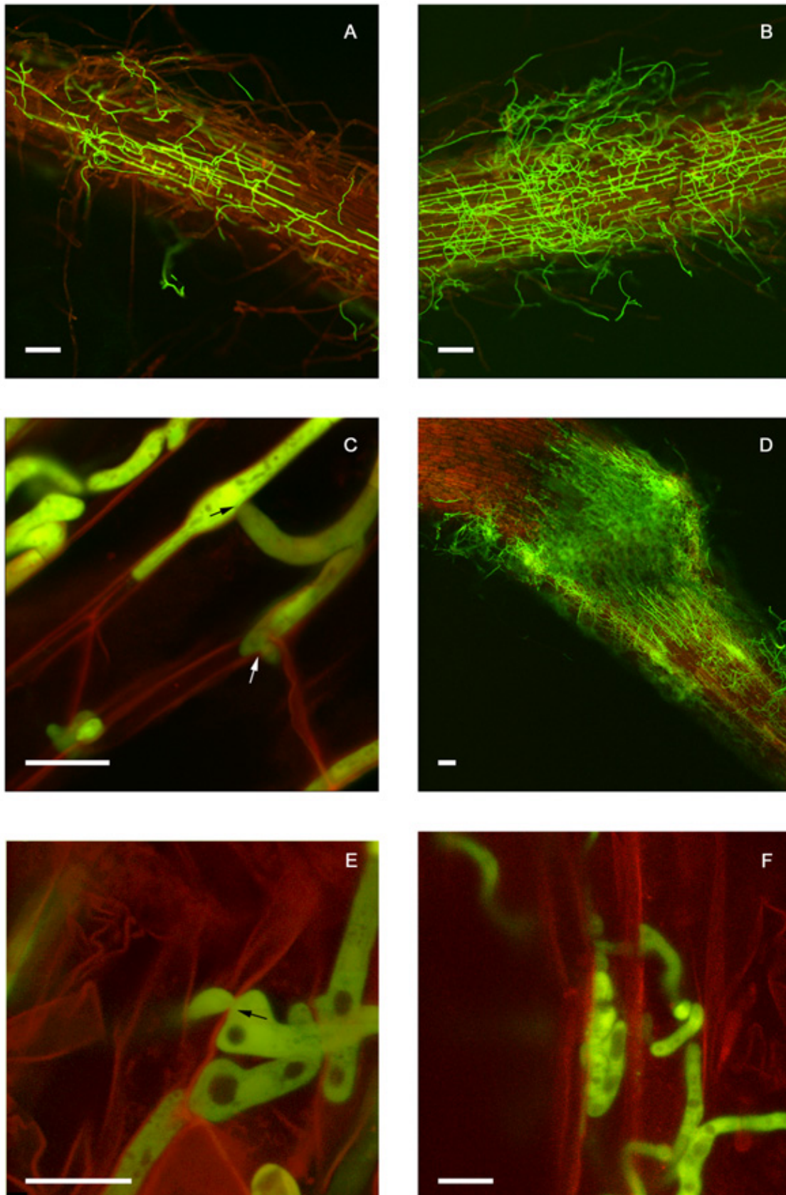
Fig. 3. Advanced stages of tomato root colonization and several stages of infection by Fusarium oxysporum f. sp. radicis-lycopersici marked with gfp . Confocal scanning laser microscopy analyses of tomato roots grown after planting 2-day-old germinated sterile seedlings in sand containing spores of F. oxysporum f. sp. radicis-lycopersici . A and B , Two subsequent steps in root surface colonization by hyphae growing at the junctions of the epidermal cells and forming an expanding network, 4 days after inoculation. C , A hypha growing at the junction of two epidermal cells, penetrating one of them (black arrow) and advancing to an adjacent cell (white arrow), 4 days after inoculation. D , Fully colonized crown of a seedling that exhibits crown rot symptoms, 4 days after inoculation. E , Intracellular growth of hyphae in root cells with a clearly visible penetration pore (indicated by arrow), 4 days after inoculation. F , Hyphae growing in epidermal root cells, 5 days after inoculation. A, B, and D , Scale bar = 50 μm and C, E, and F , scale bar = 10 μm.
