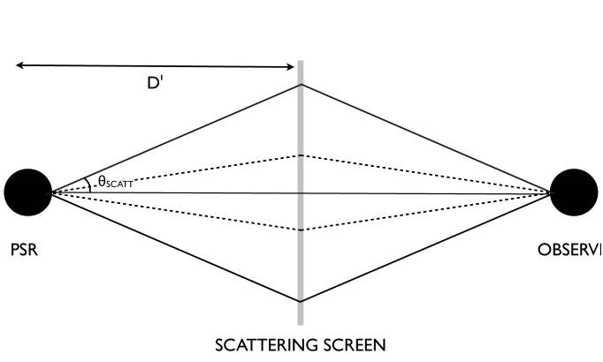
Fig. 7. The size of the scattering cone is larger at low frequencies (dark line) than at high frequencies (dashed line). The DM is a flux-weighted average over the area of the scattering disk so it varies with frequency as the scattering cone changes size.
