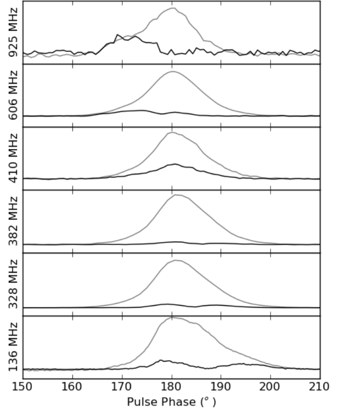
Fig. 13. Linear polarisation profiles of PSR B0809+74 between 925 and 328 MHz (Gould & Lyne 1998; Edwards & Stappers 2003b), and LOFAR polarisation profile at 136 MHz (black lines) plotted along with the Stokes I profiles at each frequency (grey lines). The polarised component moves from the position of the leading component of the profile towards later pulse longitudes, tracing the broad component of the pulse profile.
