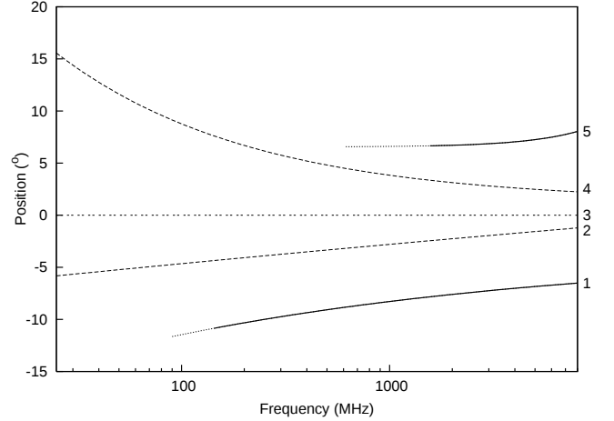
Fig. 10. A fit to the relative positions of the components of PSR B0329+54, which show a lot of asymmetry. The outer cone (bold line) is skewed towards earlier pulse longitudes and both of its components fade at very different rates. The inner cone (dashed line) is skewed in the opposite direction and again shows different spectral indices for each side of the cone. Models are less reliable in the LBAs ( < 100 MHz) where the pulse profile is affected by scattering.
