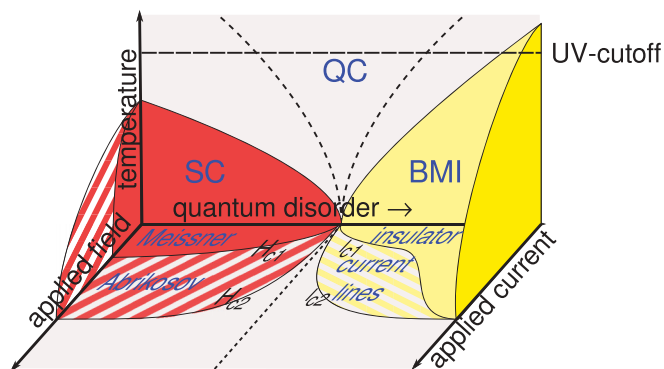
FIG. 4. (Color online) Topology of the phase diagram of type-II Bose-Mott insulators in three space dimensions. The horizontal axis represents strength of quantum phase fluctuations that tune from superconducting (SC) to Bose-Mott insulating (BMI) order via a quantum phase transition. As a function of temperature (vertical axis), the “wedge” of quantum critical fluid (QC) emerges from the quantum critical point, while on either side thermal phase transitions occur, obviously to a superconducting state, but duality also predicts a thermal transition on the insulating side. An external magnetic field is first expelled by the superconductor (Meissner), while above H_{c1} it penetrates as an Abrikosov lattice of quantized flux lines. Near the quantum phase transition, a similar response is observed in the Mott insulator, now as function of applied electric current. First, the current is expelled, just an insulator. However, above a “lower critical current” I_{c1} current will penetrate as an “Abrikosov lattice” of lines carrying a quantized current flux: the type-II Mott insulator. Upon increasing the local repulsions, one eventually enters the regime of nearly completely localized bosons. Here, the type-II Mott insulator disappears because the relevant length scales have shrunk beyond the lattice constant, the reason the type-II phase has hitherto been overlooked.
