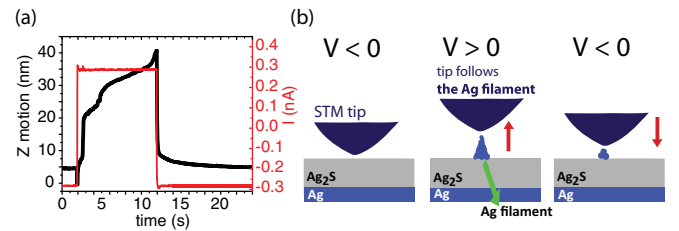
FIG. 2. (Color online) (a) Z piezodisplacement (black curve) and tunneling current (red curve) as a function of time. The growth of the Ag cluster was activated with +20 mV bias. Keeping the feedback on allows us to follow the growth of the cluster in the Z direction. (b) Schematic of the filament growth on the surface of the Ag 2 S sample.
