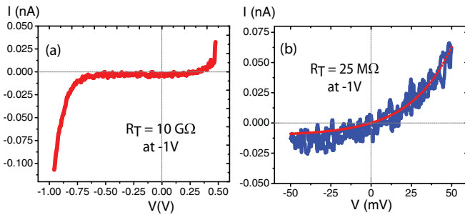
FIG. 1. (Color online) Current-voltage characteristics of the Ag 2 S thin film at two different tunneling gaps. (a) At 10 GΩ (tunneling gap defined at −1 V), the IV curve indicates the presence of the band gap in the Ag 2 S sample. (b) At 25 MΩ (tunneling gap defined at −1 V), the IV curve shows an exponential increase in the current at positive bias, due to the accumulation of Ag close to the tip for close proximity of the tip to the sample. The red curve is a fit of the IV curve from which we calculate the effective top contact radius as 0.8 nm.
