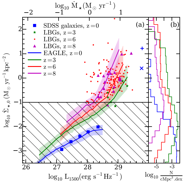
Figure 1. The dependence of the mean surface density of star formation, \Sigma_{*,0} , on star formation rate and redshift. Panel a: \Sigma_{*,0} of EAGLE galaxies with stellar mass > 10^8 M_{\odot} , as a function of their 1500 Å ultraviolet (UV) luminosity ( L_{1500} , bottom axis, corresponding star formation rate, \dot{M}_{*} , top axis), with coloured lines depicting the median relation, and coloured regions enclosing the 25th to 75th percentile range. Different colours refer to different redshifts (blue, z = 0 , green, z = 3 , red, z = 6 , magenta, z = 8 ). \Sigma_{*,0} increases with \dot{M}_{*} at given z , and with z at given \dot{M}_{*} . Horizontal black line shows the critical star formation rate surface density ( \Sigma_{*,\text{crit}} ) for outflows (Heckman 2001). Panel b: Number density of EAGLE galaxies in bins of \Sigma_{*,0} , using the same colour scheme. At z = 0 , galaxies with \Sigma_{*,0} \gtrsim \Sigma_{*,\text{crit}} above which significant winds develop are present in the simulation, but they are very rare. However at z \gtrsim 6 , most EAGLE galaxies with \dot{M}_{*} > 1 M_{\odot} \text{ yr}^{-1} are above this limit, and are expected to drive strong winds. Observed values of \Sigma_{*,0} are plotted in panel a, with colours depending on z matching those of the simulation; the region of low \Sigma_{*,0} where winds are not expected is hashed. The data shown are z = 0 , Sloan Digital Sky Survey measurements (Brisbin & Harwit 2012, squares), the galaxies with high values of f_{\text{esc}} from (Borthakur et al. 2014, cross) and (Izotov et al. 2016, plus), Lyman-break galaxies from Giavalisco, Steidel & Macchetto (1996) at z = 3 (stars), from Curtis-Lake et al. (2016) at z = 6 (small dots) and at z = 8 (triangles). EAGLE galaxies reproduce the dependence of \Sigma_{*,0} on \dot{M}_{*} and z .
