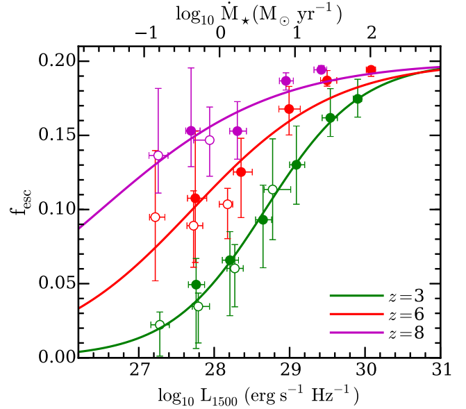
Figure 2. Mean inferred escape fraction for ionizing photons ( f_{\text{esc}} ) from galaxies in EAGLE as a function of the 1500 Å luminosity ( L_{1500} ) at three redshifts (green: z=3 , red: z=6 , magenta: z=8 ), for f_{\text{esc,max}} = 0.2 . Circles represent the luminosity-weighted average of f_{\text{esc}} , with error bars encompassing the 25th to 75th percentile range. Filled circles refer to the reference simulation (labelled Ref-L0100N1504), open circles to the simulation that has eight times better mass resolution (labelled Recal-L0025N0752). Simulation results are fitted with a sigmoid function shown as solid curves. The escape fraction increases with luminosity and redshift.
