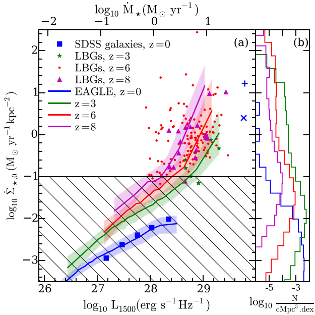
Figure 1. The dependence of the mean surface density of star formation, \Sigma_{*,0} , on star formation rate and redshift. Panel a: \Sigma_{*,0} of EAGLE galaxies with stellar mass > 10^8 \text{ M}_\odot , as a function of their 1500 Å ultraviolet (UV) luminosity ( L_{1500} , bottom axis, corresponding star formation rate, \dot{M}_* , top axis), with coloured lines depicting the median relation, and coloured regions enclosing the 25th to 75th percentile range. Different colours refer to different redshifts (blue, z=0 , green, z=3 , red, z=6 , magenta, z=8 ). \Sigma_{*,0} increases with \dot{M}_* at given z , and with z at given \dot{M}_* . Horizontal black line shows the critical star formation rate surface density ( \Sigma_{*,\text{crit}} ) for outflows (Heckman 2001). Panel b: Number density of EAGLE galaxies in bins of \Sigma_{*,0} , using the same colour scheme. At z=0 , galaxies with \Sigma_{*,0} \gtrsim \Sigma_{*,\text{crit}} above which significant winds develop are present in the simulation, but they are very rare. However at z \gtrsim 6 , most EAGLE galaxies with \dot{M}_* > 1 \text{ M}_\odot \text{ yr}^{-1} are above this limit, and are expected to drive strong winds. Observed values of \Sigma_{*,0} are plotted in panel a, with colours depending on z matching those of the simulation; the region of low \Sigma_{*,0} where winds are not expected is hashed. The data shown are z=0 , Sloan Digital Sky Survey measurements (Brisbin & Harwit 2012, squares), the galaxies with high values of f_{\text{esc}} from (Borthakur et al. 2014, cross) and (Izotov et al. 2016, plus), Lyman-break galaxies from Giavalisco, Steidel & Macchetto (1996) at z=3 (stars), from Curtis-Lake et al. (2016) at z=6 (small dots) and at z=8 (triangles). EAGLE galaxies reproduce the dependence of \Sigma_{*,0} on \dot{M}_* and z .
