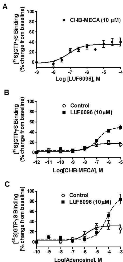
Fig. 4. Effect of LUF6096 on [ ^{35} S]GTP \gamma S binding in assays with the canine A_3 AR. Incubations were started by the addition of the membrane suspension (5 \mu g of protein) as described under Materials and Methods and carried out in quadruplicate for 2 h at 25°C. The membrane solutions were preincubated with LUF6096 for 30 min at 25°C before the addition of \sim 0.1 nM [ ^{35} S]GTP \gamma S. A, the effect of increasing concentrations of LUF6096 on [ ^{35} S]GTP \gamma S binding in response to a maximal concentration of Cl-IB-MECA ( 10^{-5} M) ( n = 9 ). B, stimulation of [ ^{35} S]GTP \gamma S binding by increasing concentrations of Cl-IB-MECA in the absence (control) or presence of LUF6096 (10 \mu M) ( n = 6 ). C, stimulation of [ ^{35} S]GTP \gamma S binding in response to increasing concentrations of adenosine in the absence (control) or presence of LUF6096 (10 \mu M) ( n = 5 ).
