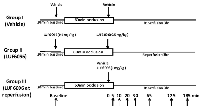
Fig. 2. Schematic illustration of the experimental protocols. The arrows to the right in the protocol for group III indicate the time after drug administration that blood samples were collected from the femoral vein for determination of the plasma concentration of LUF6096.
