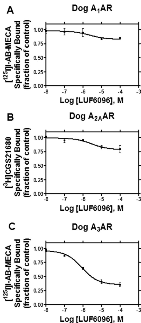
Fig. 5. Effect of LUF6096 on equilibrium orthosteric radioligand binding to the canine A_1 (A), A_{2A} (B), and A_3 (C) ARs. Membranes (50 \mu g) were incubated with [ ^{125} I]I-AB-MECA ( \sim 0.5 nM; A_1 and A_3 ARs) or [ ^3 H]CGS21680 ( \sim 10 nM; A_{2A} ARs) for 2 h at room temperature in the presence of increasing concentrations of LUF6096. Nonspecific binding was determined with 200 \mu M adenosine-5'-N-ethylcarboxamide. The data shown are representative of three independent experiments.
