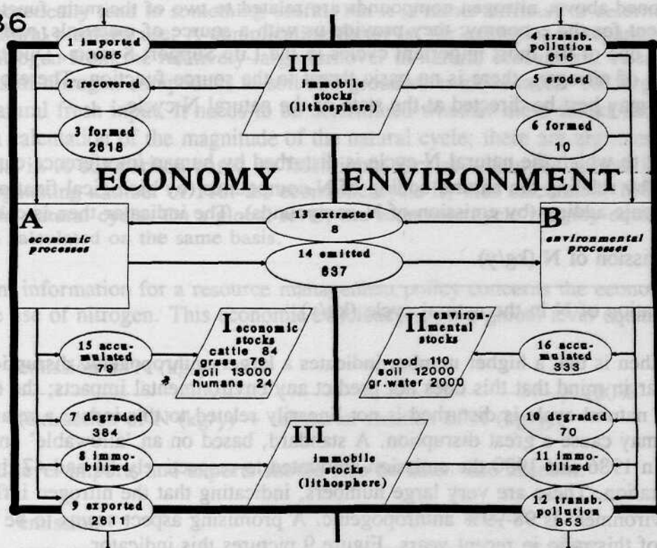
Figure 8 Balances of nitrogen compounds in The Netherlands in 1986 and 1990. Based on CBS balances (Olsthoorn, 1989 and Olsthoorn, 1993). Numbers in \text{kg} \cdot 10^6 \text{ N/year} .
