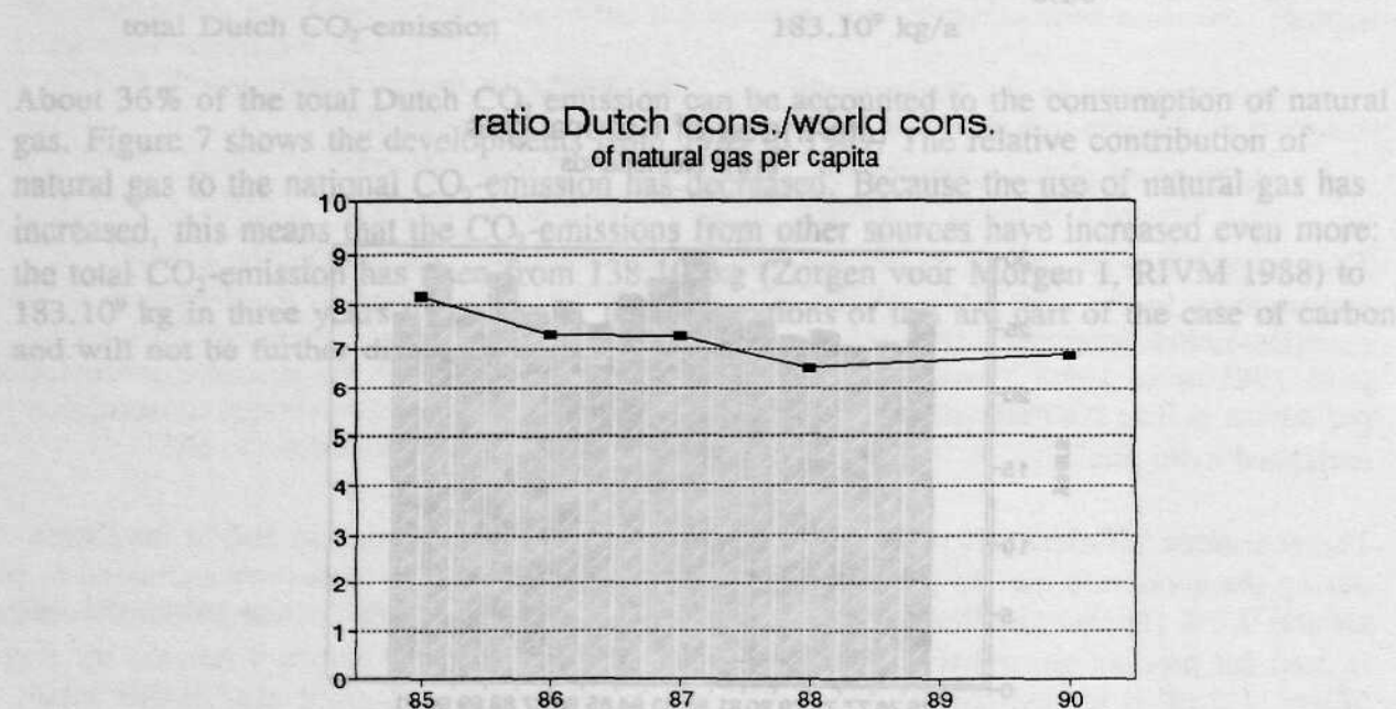
Figure 6 The Netherlands contribution to the consumption of natural gas per capita. Sources: CBS, 1993 and United Nations Energy Statistics Yearbook.
