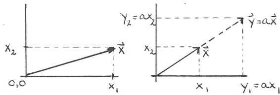
6A: vector \vec{x}
