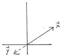
8B: collinear - b < 0
