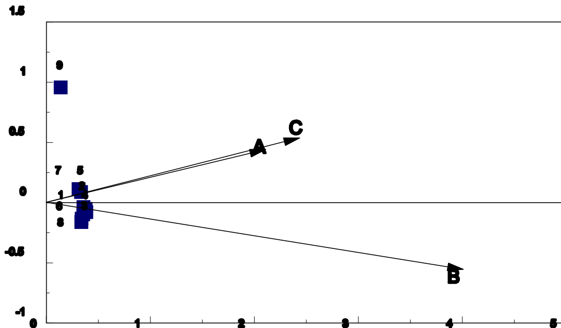
Figure 2 Biplot of the perfectly two-dimensional raw data (Note: The scaling of the horizontal and vertical axes is not equal).
