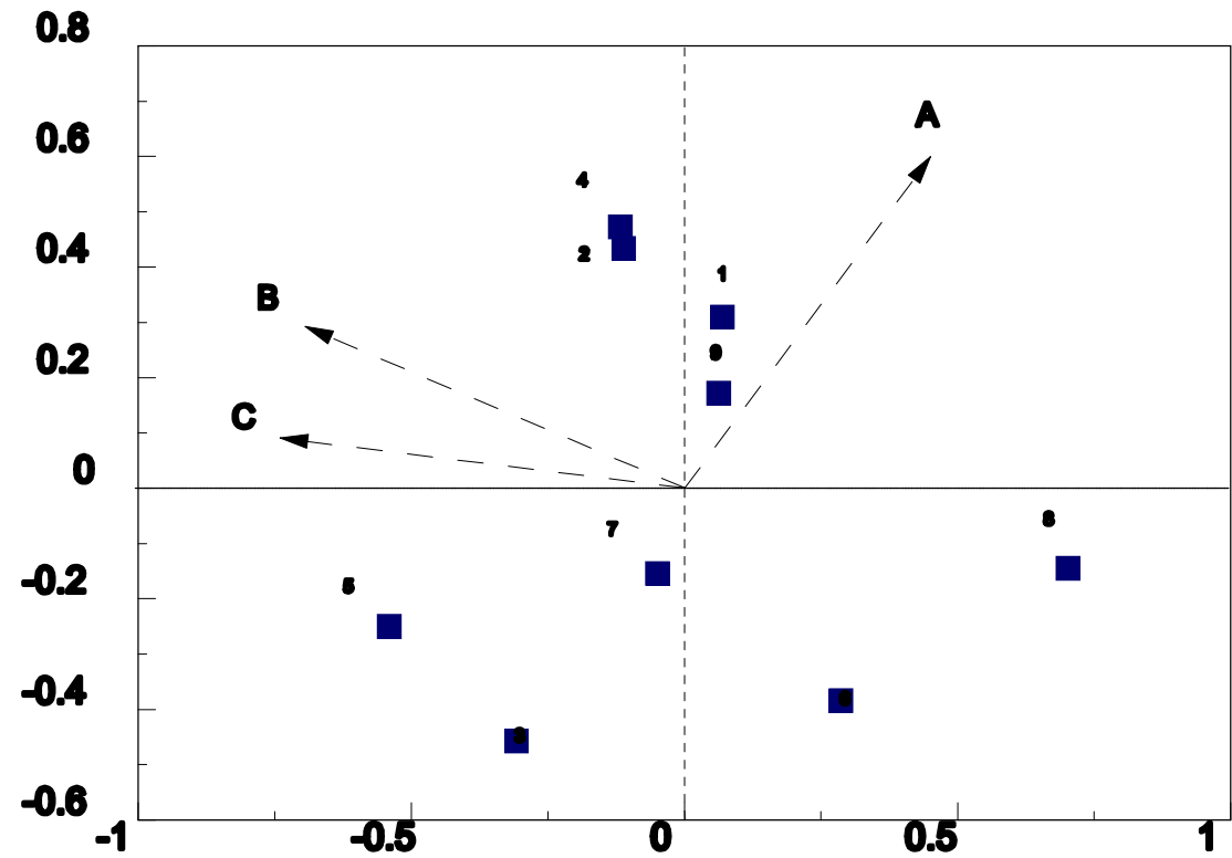
Figure 4 Biplot of the perfectly two-dimensional environment standardised data.
