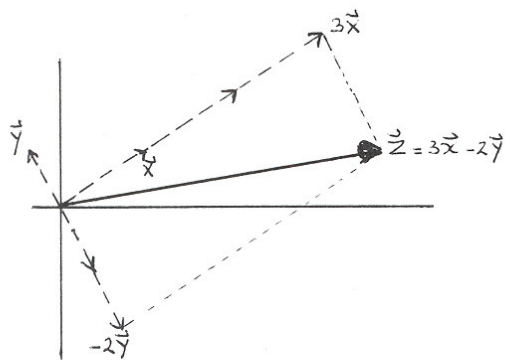
7A: linear combination
