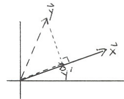
8D: projection of \vec{y} on \vec{x}
