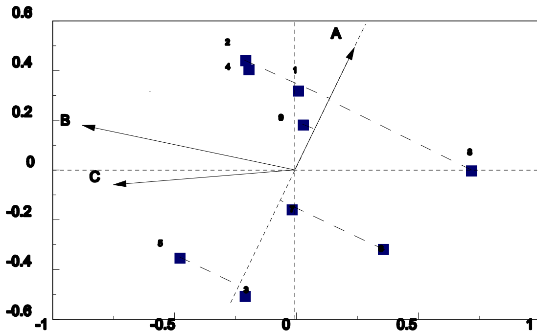
Figure 3 Biplot for the perfectly two-dimensional centred data
