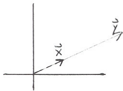
8A: collinear - b > 0
