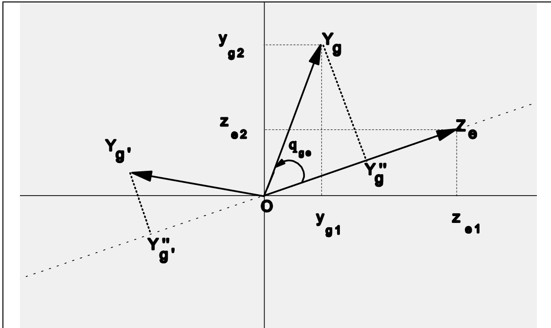
Figure 1 Representation of two genotype markers and one environment marker in a biplot.
