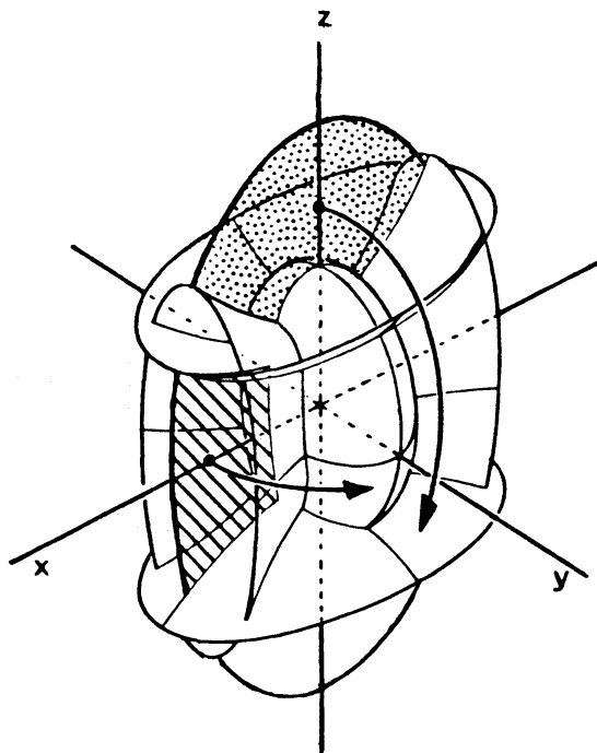
Figure 3. Shapes of two possible three-dimensional orbits in a Stäckel potential. An orbit in the volume bounded by coordinate surfaces that is obtained by taking the dashed area around the z -axis, as indicated by the arrow, is a short axis tube orbit. An orbit in the volume that is obtained by taking the dotted area around the x -axis in a similar way is an outer long axis tube orbit.
