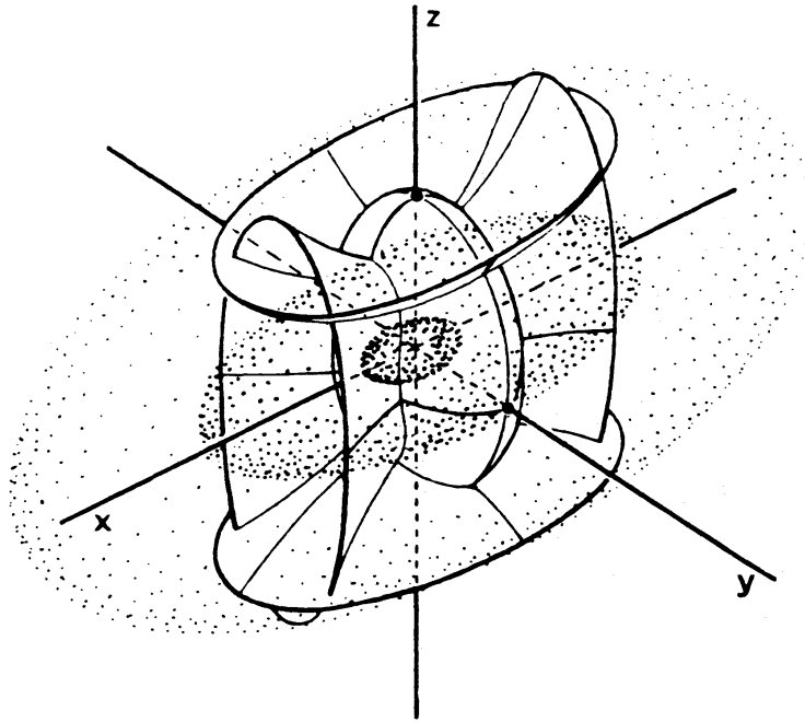
Figure 1. Ellipsoidal coordinates (\lambda, \mu, \nu) . The coordinate surfaces are ellipsoids and hyperboloids of one and two sheets. The density corresponding to a potential of Stäckel form in these coordinates is indicated.
