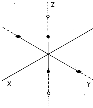
Figure 4. Axial orbits and their stability in a three-dimensional Stäckel potential. The filled squares and the filled and open circles denote the foci. A dashed line indicates orbits that are unstable in one direction; a dotted line indicates the z -axis orbits that are unstable in two perpendicular directions.
