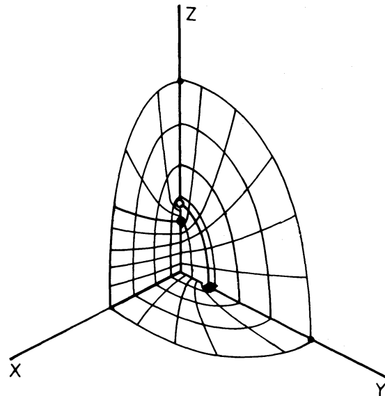
Figure 2. In each principal plane the ellipsoidal coordinates are elliptic coordinates.
