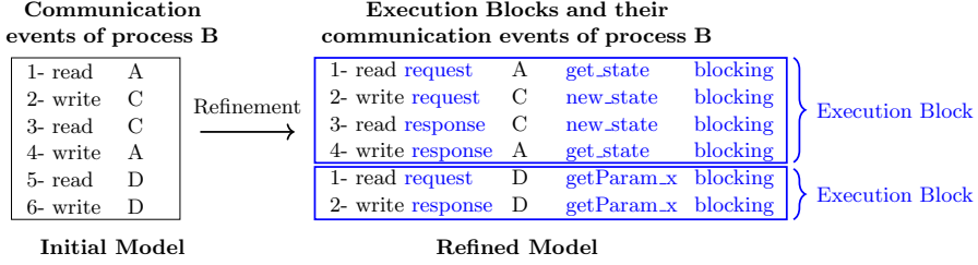
Figure 6.3: Refinement of the application workload model
