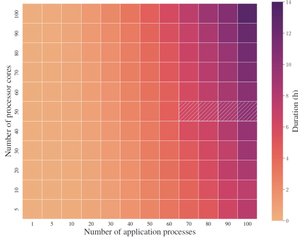
Figure 2.2: Heatmap of the DSE runtime (in hours) by varying the number of application processes and processing components
