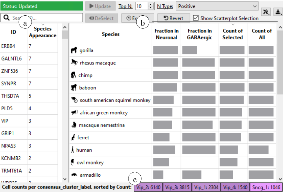
Figure 3.4: Table view for cell type abundance and gene expression exploration. The left panel (a) is gene-focused and lists all genes that are marker gene candidates in at least one species; the right panel (b) is focused on species and used for detailed analysis of cell abundance and differential expression. The bottom row (c) shows the distribution of the selected cells across different cell types.
