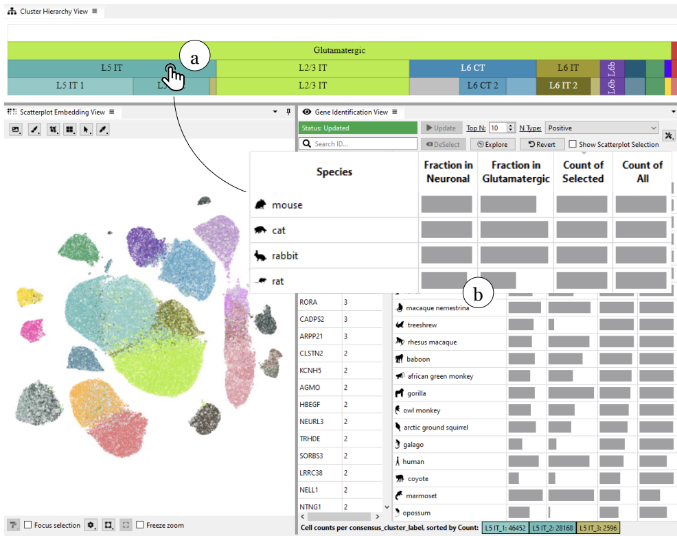
Figure 3.8: The first step in the case study is to identify the L5IT cells in the cell type hierarchy (a), select it, and explore the corresponding abundances in the detail table view (b).
