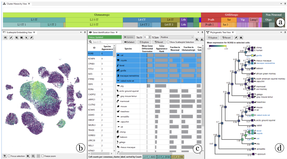
Figure 3.1: Cytosplore EvoViewer showing data on cell composition within the primary motor cortex of twenty-five mammalian species with four views: cell type hierarchy (a), single-cell embedding (b), detail table (c), and phylogenetic tree (d).
