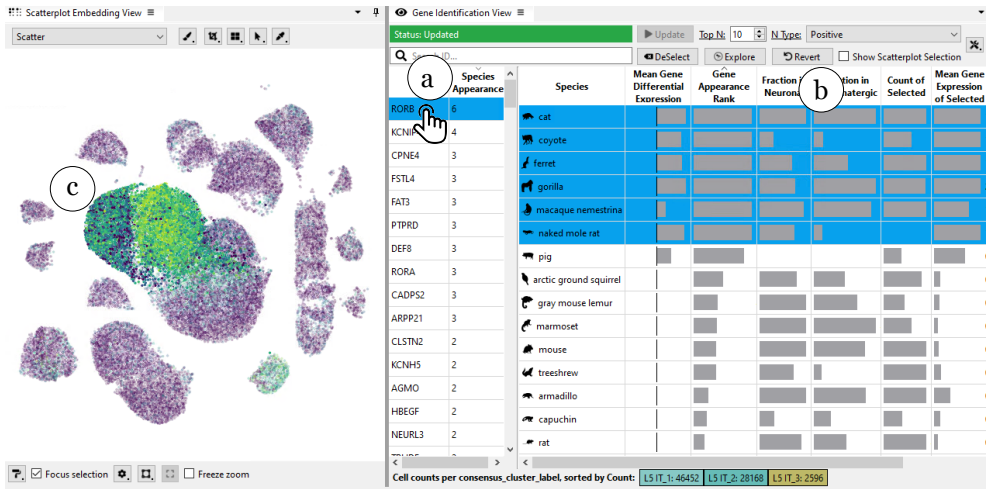
Figure 3.9: Inspecting table view for the selected RORB gene (a) reveals six species for which the gene ranks as a potential marker gene for L5IT (b). The UMAP embedding (c) shows high expression for those species in a confined area, comprising L5IT cells.
