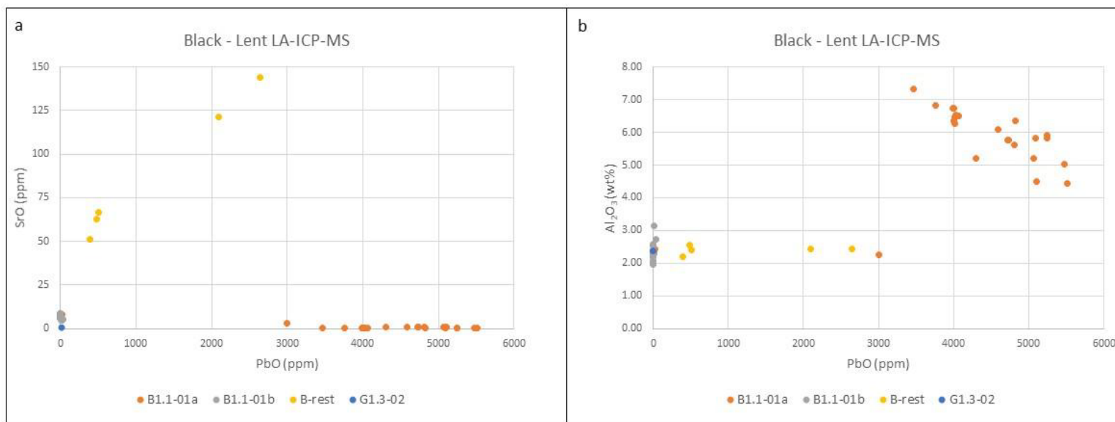
Fig. 4.9 Chemical composition of black beads: a) Biplot black beads PbO vs SrO plotted per main bead-type (LA-ICP-MS). b). Biplot black beads PbO vs AlO plotted per main bead-type (LA-ICP-MS).
