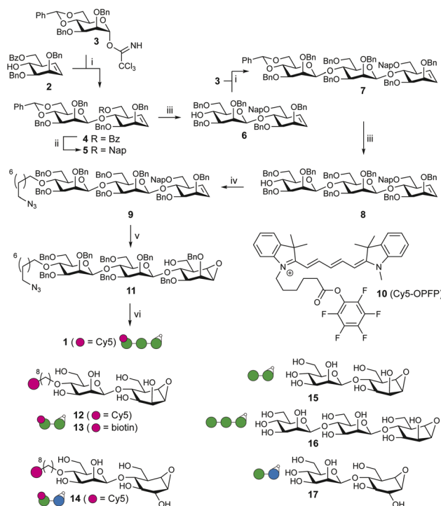
Scheme 1 Inhibitor and probe design and synthesis of ABP 1 . Reagents and conditions: (i) TMS-OTf, \text{CH}_2\text{Cl}_2 , -45^\circ\text{C} (95% 4 , 99% 7 ); (ii) (a) NaOMe, MeOH/ \text{CH}_2\text{Cl}_2 (89%); (b) NapBr, NaH, TBAI, DMF (71%); (iii) CSA, MeOH, 50^\circ\text{C} , then 2-aminoethyl diphenylborinate, BnBr, KI, \text{K}_2\text{CO}_3 , \text{CH}_3\text{CN} (74%, 81% 8 ); (iv) 1-azido-8-iodooctane, NaH, DMF (77%); (v) DDQ, \text{CH}_2\text{Cl}_2/\text{H}_2\text{O} (83%), then mCPBA, \text{CH}_2\text{Cl}_2 , 0^\circ\text{C} (83%); (vi) Na, \text{NH}_3 , t -BuOH, THF, -60^\circ\text{C} (16%), then Cy5-OPFP 10 , DiPEA, DMF (99%).
