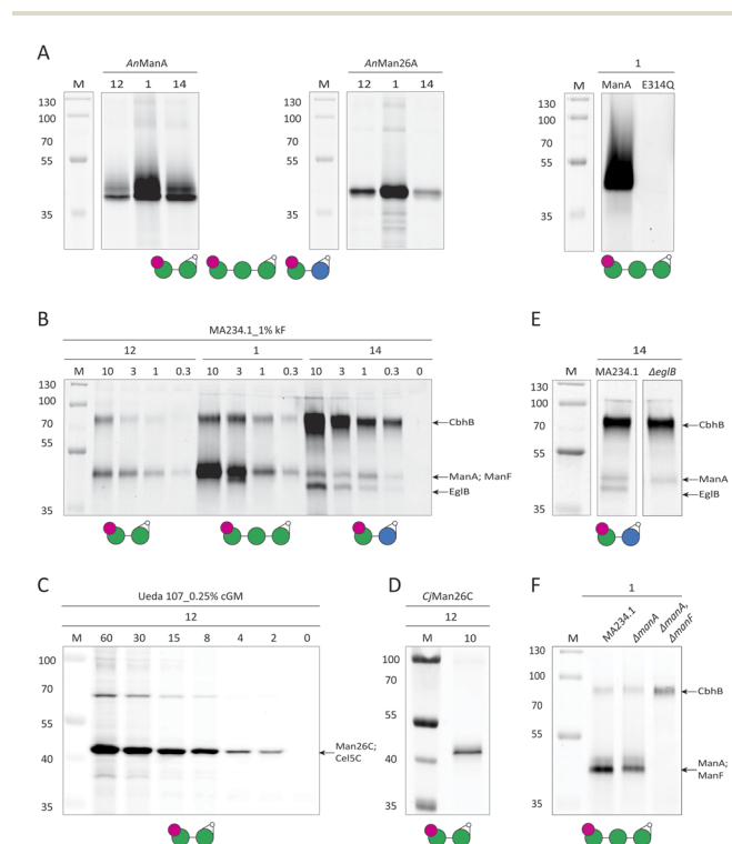
Fig. 2 (A) Labelling of recombinant A. niger mannanases An ManA, An Man26A with 1 , 12 and/or 14 and labelling with 1 of the secretomes of A. niger strains overexpressing either ManA or its E314Q mutant. (B) Comparative ABPP using ABPs 1 , 12 and 14 at 0 to 10 \mu M final concentrations on secretomes of A. niger MA234.1 cultured on konjac flour (kF). (C) Comparative ABPP with 12 at 0 to 60 \mu M final concentrations of lysate of C. japonicus Ueda 107 grown on carob galactomannan (cGM). (D) Labelling of recombinant C. japonicus mannanase Cj Man26C with 12 . (E) ABP labelling with 14 of the secretomes of the A. niger strains MA234.1 and \Delta eglB grown on kF for 72 h. (F) Labelling with ABP 1 of the secretomes of A. niger MA234.1, \Delta manA and \Delta manF grown on kF for 72 h.
