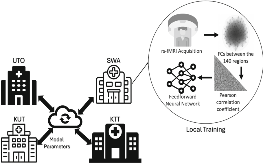
Fig. 1. Proposed TVFed-P framework.
