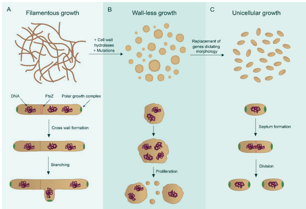
Figure 3. Proposed innovative approach for morphology engineering of streptomycetes via L-forms. Morphology of a filamentous streptomycete and its normal mode of growth (A). Without their cell wall, spherical cells are obtained that proliferate without the canonical cell division machinery as so-called L-forms (B). These L-forms offer an innovative avenue for strain engineering, wherein the entire cell division apparatus can be substituted, such as with that of the unicellular bacterium Corynebacterium . This process holds the potential to create a unicellular Streptomyces strain (C).
