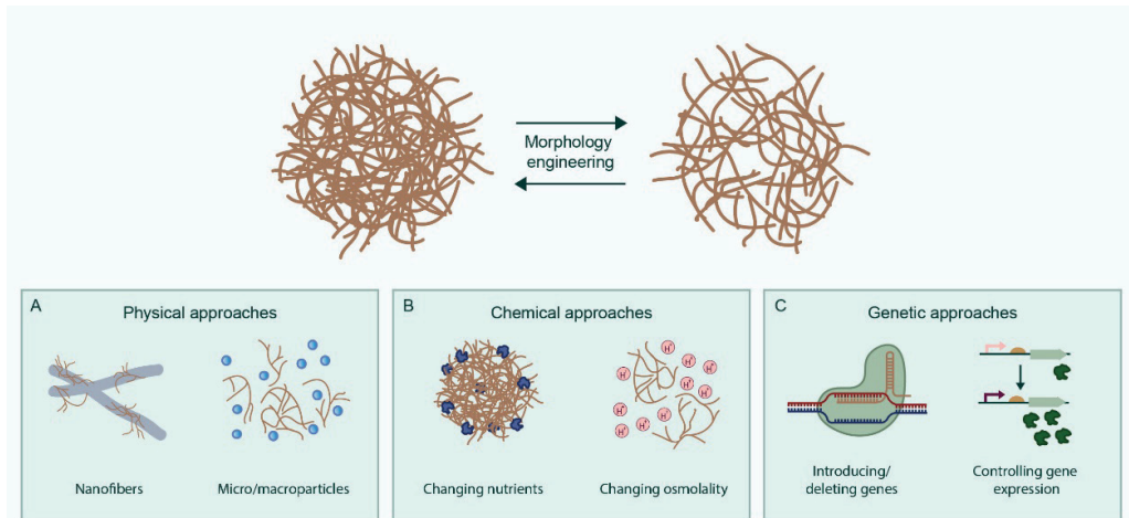
Figure 2. Overview of the three central approaches to engineer the morphology of multicellular bacteria. Physical approaches include the use of nanofibers and micro- and macroparticles (A). Chemical approaches include changing nutrients and medium osmolality (B). Genetic approaches include deleting and introducing genes and controlling gene expression (C).
