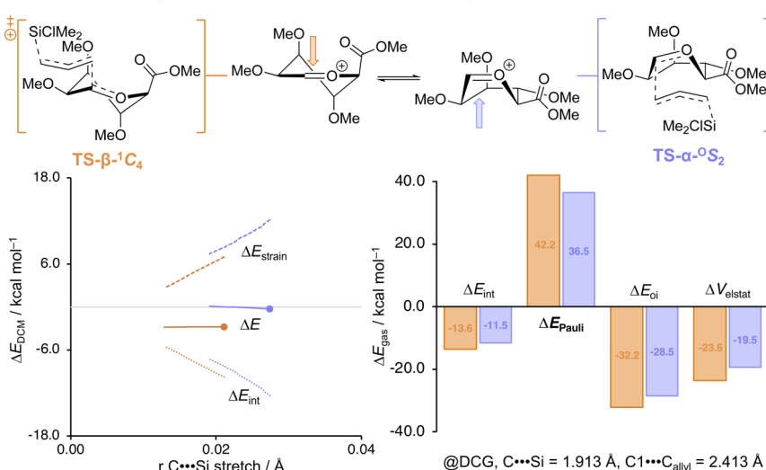
Fig. 4 Activation strain and energy decomposition analyses for the S_N2' reactions of allyl (chloro)dimethylsilane and the (A) rhamnosyl cation and (B) the mannanosyl cation via the \beta -product-forming TS- \beta^1\text{C}_4 (orange) and the \alpha -product-forming TS- \alpha\text{-OS}_2 (light violet). Energy values are plotted to the transition state (indicated by a dot), along the IRC projected on the C \cdots Si bond stretch. Energies are depicted as electronic energies and were computed at PCM(CH _2 Cl _2 )-B3LYP/6-311G (d,p) for \Delta E_{\text{DCM}} or ZORA-B3LYP/TZ2P//PCM(CH _2 Cl _2 )-B3LYP/6-311G (d,p) for \Delta E_{\text{gas}} .
