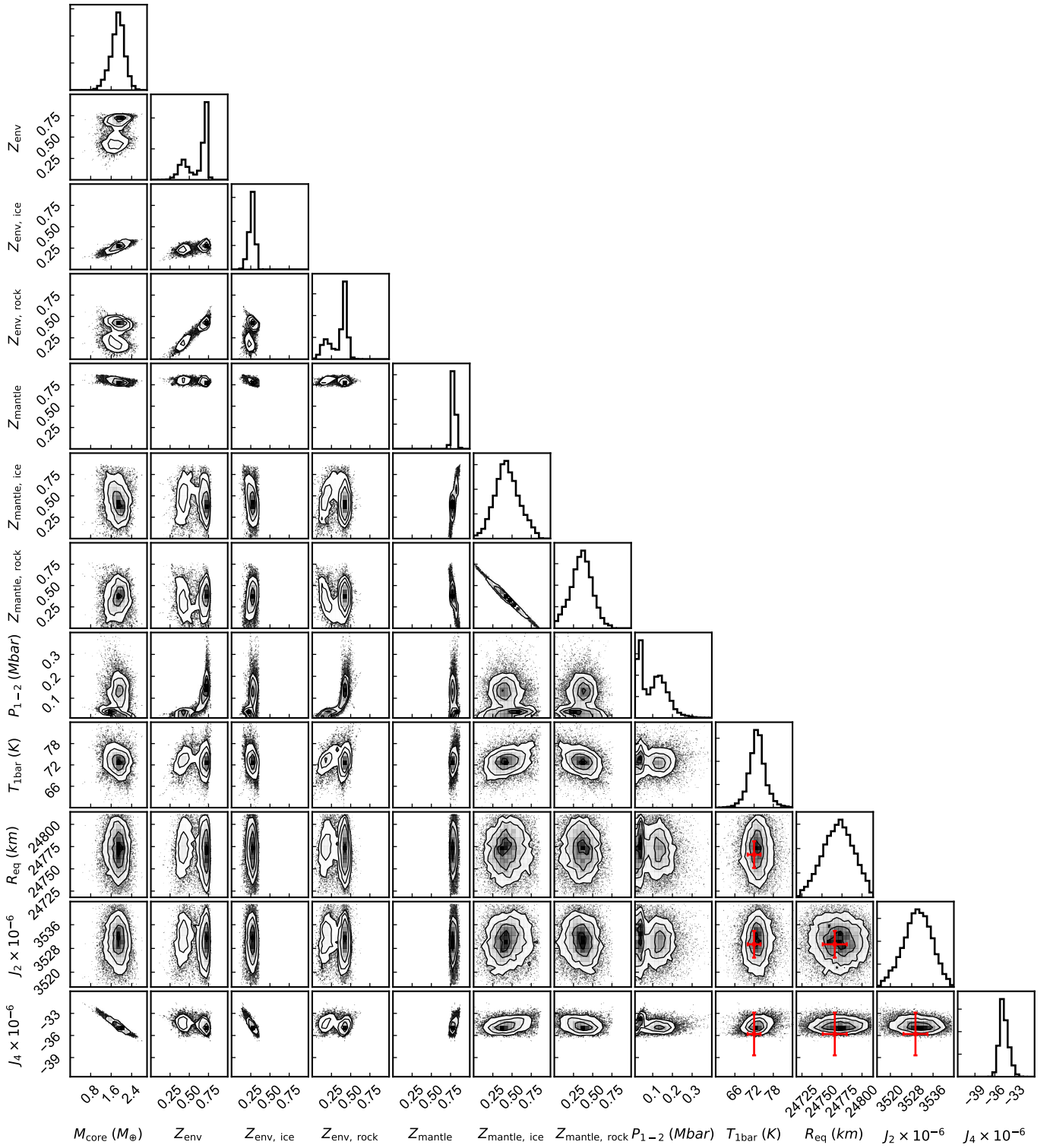
Fig. B.3: Same as Fig. B.1 but for the alternative ice+rock model of Neptune, adopting REOS for water and QEOS for \text{SiO}_2 for the rocky component.
