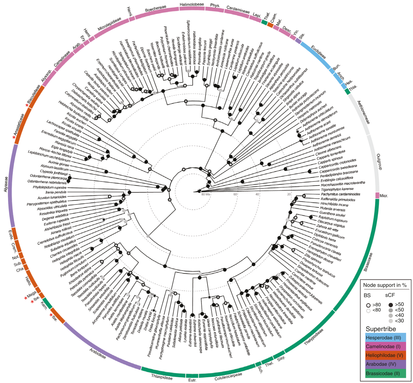
FIG. 2. Time-calibrated genus-level mitogenomic Brassicaceae phylogeny based on the ‘selective’ strategy, from a maximum likelihood approach analysis of 32 mitochondrial genetic markers. Node support is indicated by circles, with outer circles representing bootstrap (BS) values and inner circles representing site concordance factors (sCF). Supertribes are colour-coded, and red asterisks mark rogue taxa (as defined by German et al. , 2023; Hendriks et al. , 2023; see also Table 2). Tribe names are given along the outer edge of the phylogeny. For a richly annotated and detailed version, see Supplementary Data Fig. S2. Abbreviations of tribes are as follows: Anch., Anchonieae; Arab., Arabidopsidae; Bun., Buniadeae; Cha., Chamireae; Crem., Cremolobae; Desc., Descurainiae; Ery., Erysimeae; Eude., Eudemeae; Eutr., Eutremeae; Helio., Heliophleae; Hemi., Hemilophleae; Hes., Hesperideae; Ibe., Iberideae; Lepi., Lepidideae; Mal., Malcolmiae; Mega., Megacarpaceae; Micr., Microlepidideae; Not., Notothlaspidiae; Phys., Physarieae; Ste., Stevenieae; Sub., Subularieae; Thel., Thelypodieae; Thla., Thlaspidiae; Yn., Yinshanieae.
