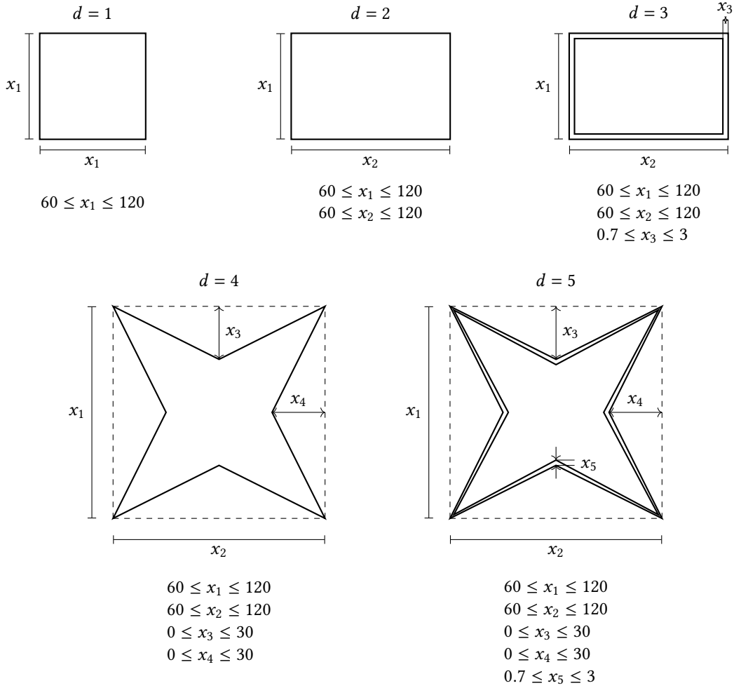
Fig. 4. Optimization problem parameterization for d \leq 5 . The ranges of each variable are expressed in mm. The drawings are not in scale. For the cases where thickness is not controlled such as the cases where d = \{1, 2, 4\} , the wall thickness t_h is set constant to 2.1 mm.
