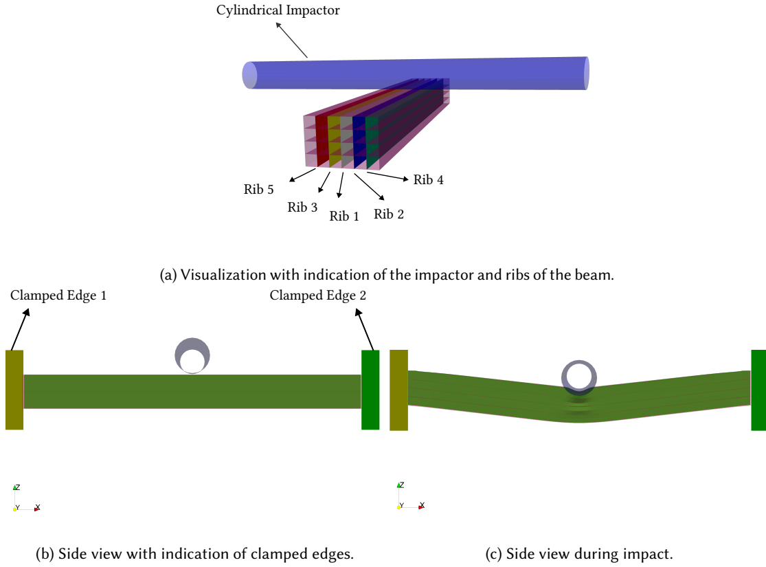
Fig. 6. Representation of the Three Point Bending of Layered Beam case.
