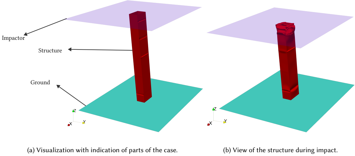
Fig. 9. Representation of the Long Crash Tube Case.
