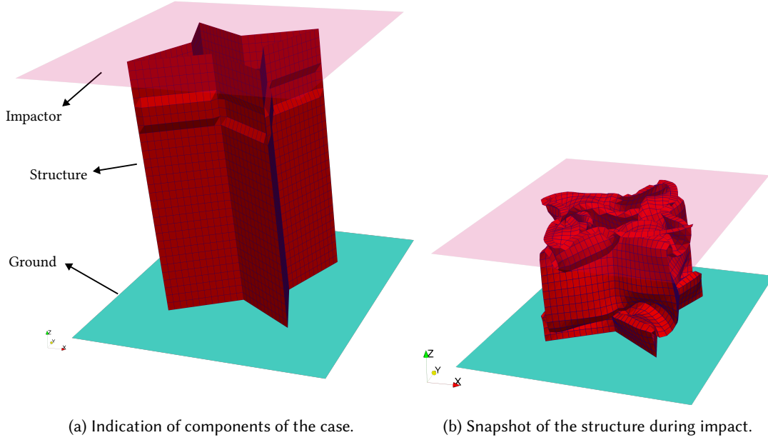
Fig. 3. Star-shaped crash-box case. The structure is subdivided into smaller connected parts, forming a finite element mesh shown by the blue lines. In the z -direction, the mesh is arranged in 30 rows of elements, wherein each row is assigned the same thickness value t_h .
