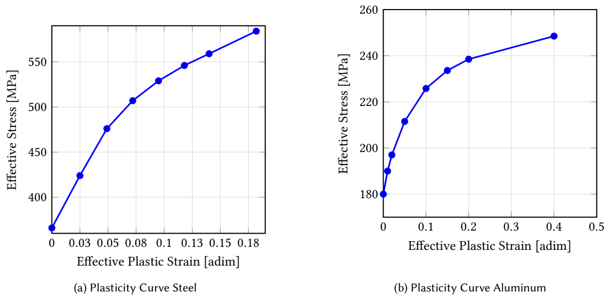
Fig. 13. Plasticity Curves used for the Material Models. Adapted from Kaps et al. [20].
