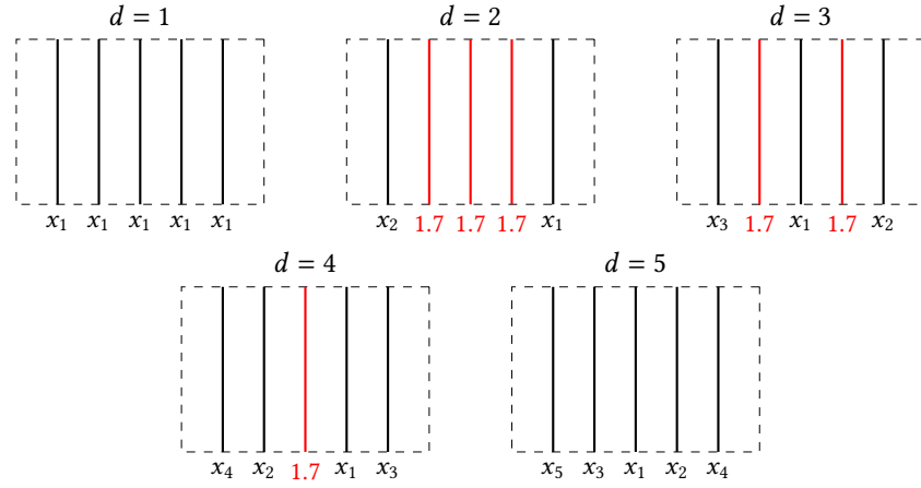
Fig. 7. Optimization problem parameterization for d \leq 5 . Each variable is expressed in mm. In red are the ribs which have a predefined thickness of 1.7 mm. Each line is annotated by the design variable denoting the wall thickness of the respective rib.
