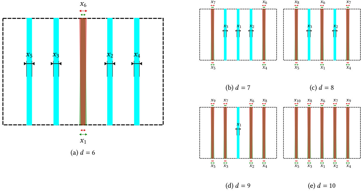
Fig. 8. Description of point addition used to develop wall thickness profiles for each of the five ribs of the beam for d = 6, 7, 8, 9, 10 . For the dimensions shown, the straight rectangles colored in cyan indicate a constant thickness along the corresponding rib. In contrast, the two sets of trapezoids, colored in semi-transparent red and semi-transparent green , represent linearly increasing and decreasing thickness profiles, respectively. The superposition of these trapezoids is used to emphasize that the thickness profile of a rib may be expressed as either increasing or decreasing, depending on the variable values. For 10 < d \leq 40 , control points are added in a similar fashion as the shown sequences herein.
