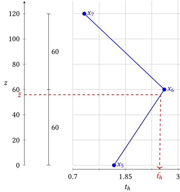
Fig. 5. Thickness distribution example for d = 7 , wherein 3 control points are set at uniformly distributed heights between 0 and 120 mm and each point has an assigned t_h(z) . The wall thickness t_h at any intermediate point \bar{z} is computed via linear interpolation of assigned t_h of the neighboring control points. This procedure is used to compute the wall thickness t_h of a row of finite elements by getting the interpolated \bar{t}_h at the element barycenter.
