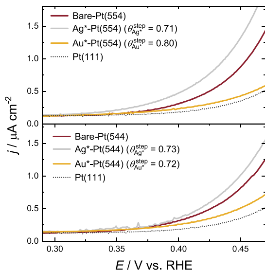
Figure 4. Linear sweep voltammograms (LSVs) of CO oxidation in CO bulk-saturated 0.1 mM \text{HClO}_4 electrolyte for (top) bare Pt(554) (brown), \text{Ag}^* -Pt(554) ( \theta_{\text{Ag}^*}^{\text{step}} = 0.71 ) (silver), \text{Au}^* -Pt(554) ( \theta_{\text{Au}^*}^{\text{step}} = 0.80 ) (gold), bare Pt(111) (black dashed) and (bottom) bare Pt(544) (brown), \text{Ag}^* -Pt(544) ( \theta_{\text{Ag}^*}^{\text{step}} = 0.73 ) (silver), \text{Au}^* -Pt(544) ( \theta_{\text{Au}^*}^{\text{step}} = 0.72 ) (gold), bare Pt(111) (black dashed), measured in 0.1 mM \text{HClO}_4 , \nu = 10 \text{ mV s}^{-1} .
