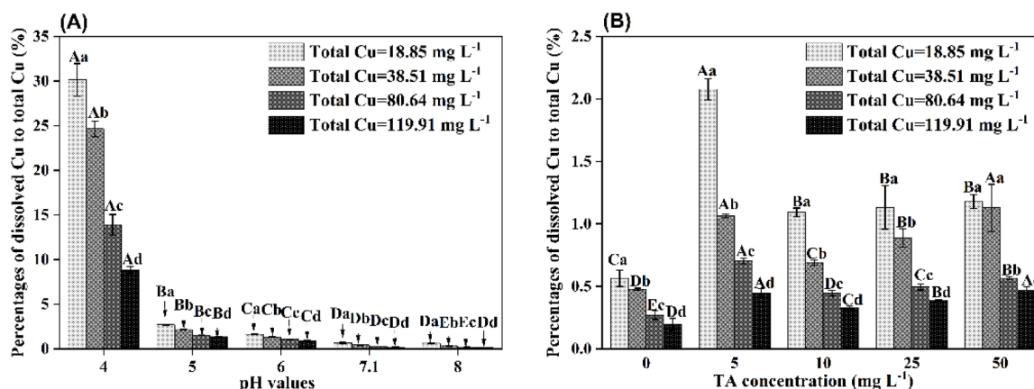
Fig. 3. Percentages of dissolved Cu in CuO NPs suspensions after 96 h exposure at various levels of pH (A) and TA (B, pH \approx 7.1). Capital letters represent the comparison between averaged dissolution percentages at the same concentration of total Cu namely intergroup comparison. Lower letters represent the comparison between averaged dissolution percentages at the same value of pH or TA namely intragroup comparison. Different letters indicate significant differences found using the One-way ANOVA test ( p < 0.05 ). Total Cu indicates the measured total concentrations of Cu in CuO NPs suspension under different treatments. Data are presented as mean \pm standard error of the mean ( n = 3 ).
