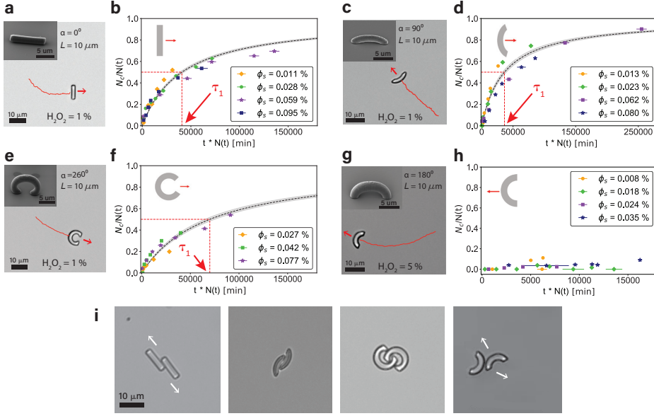
Figure 2.4: Shape-dependent clustering behavior Scanning electron microscopy (inset) and bright-field images of 3D printed (a) straight rods ( \alpha = 0^\circ ), (c) \alpha = 90^\circ , (e) \alpha = 260^\circ and (g) \alpha = 180^\circ . The trajectory travelled by the active particle in the past 30 s is shown in red and the direction of motion is indicated by a red arrow. Fraction of particles in a cluster plotted after rescaling time as t \rightarrow tN(t) for systems of (b) self-propelled straight rods, (d, f) concave-side leading crescents with (d) \alpha = 90^\circ and (f) \alpha = 260^\circ , and (h) convex-side leading crescents with \alpha = 180^\circ . The fit parameter obtained from fitting with Eq. (2.1) is (b) \tau_1 = (4.1 \pm 0.2)10^4 min, (d) \tau_1 = (3.6 \pm 0.3)10^4 min, and (f) \tau_1 = (7.0 \pm 0.5)10^4 min respectively. The x -error indicates the observation time needed to measure the entire sample. All surface area fractions \phi_s correspond to particle densities below 50 crescents/mm 2 . The exact values can be found in the Appendix. (i) Bright-field images of rods and crescent pairs that differ in their ability to interlock, cf. Supporting Video7-12. The white arrow indicates how pairs that are not sufficiently stabilized by interlocking can slide past each other and break. Source data are provided as a Source Data file.
