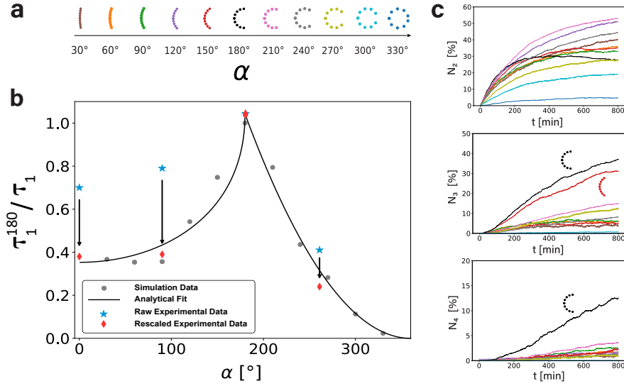
Figure 2.5: Simulation results on the influence of the opening angle \alpha on the clustering behaviour (a) Bent rods with increasing opening angle from 30^\circ to 330^\circ used in the simulations shown in (b). (b) Inverse fit parameter 1/\tau_1 as a function of the opening angle \alpha , normalized to the value of \tau_1 for \alpha = 180^\circ . The fit is found from a simple model describing cluster creation and decay, see the main text for details. The fit shown here is \tau_1^{180}/\tau_1 = 2.357(1.149 - 1/\sqrt{d(\alpha)^2 + 1})\Theta(\pi - \alpha) + 0.106P_{clu}\Theta(\alpha - \pi) , with \Theta the Heaviside step function. The red data points (star) represents the normalised inverse fit parameter for straight rods, 90^\circ crescents and 260^\circ crescents (from left to right) found in experiments before rescaling, the blue data points (diamond) the value after rescaling (see main text and Appendix). (d) Evolution over time of the number of particles in a two-particle-cluster (top-left), a three-particle-cluster (top-right) and a four-particle-cluster (bottom-left), respectively. Source data are provided as a Source Data file.
