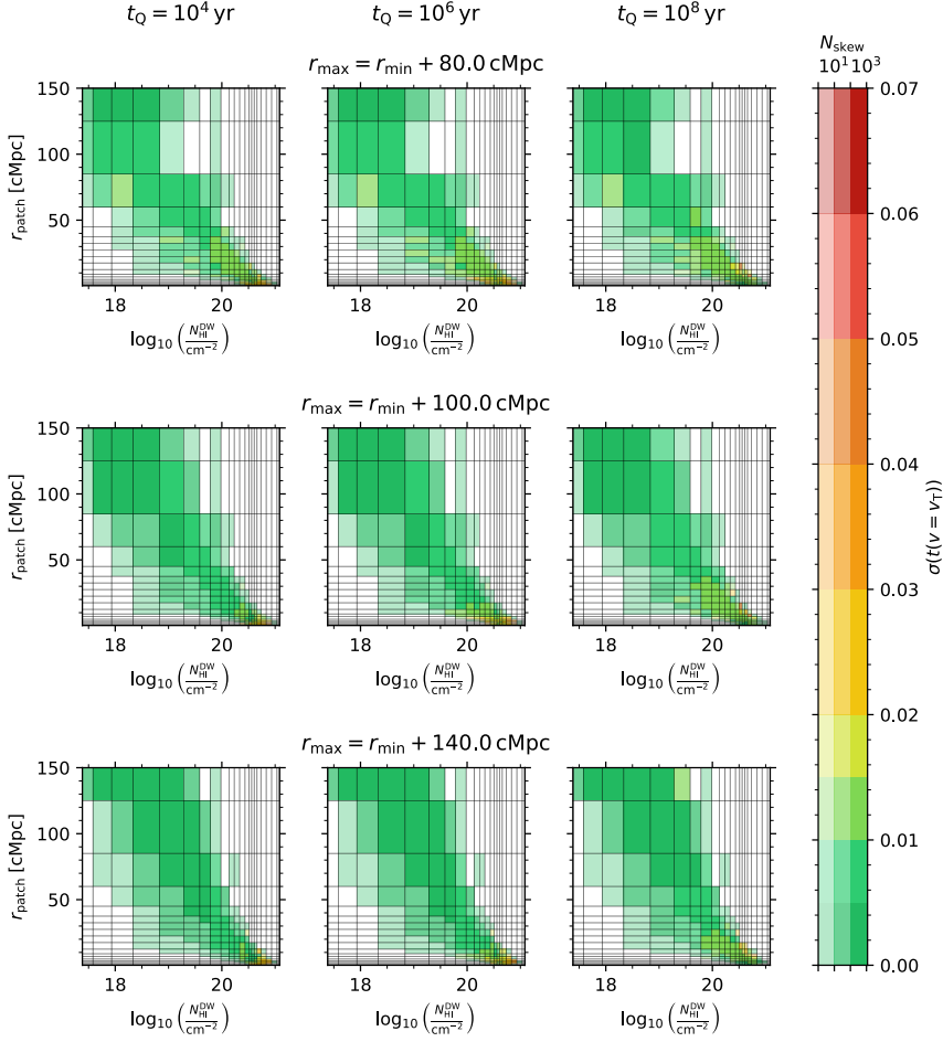
Figure 3.13: Like Figure 3.12 but for upper integration limits of r_{\text{max}} = r_{\text{min}} + 80.0 cMpc (upper row), r_{\text{max}} = r_{\text{min}} + 100.0 cMpc (middle row) and r_{\text{max}} = r_{\text{min}} + 140.0 cMpc (lower row) for the HI column density N_{\text{HI}}^{\text{DW}} .
