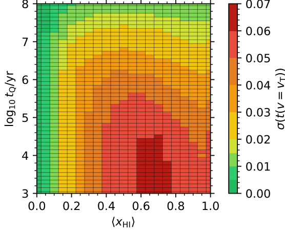
Figure 3.5: Sightline-to-sightline scatter of the IGM damping wing as a function of astrophysical parameter space in the global (\langle x_{\text{HI}} \rangle, t_Q) -parameterization. The scatter is quantified as half the 68-percentile width \sigma(t(v = v_T)) of the distribution of IGM transmission values at v = v_T among all sightlines at a given location in (\langle x_{\text{HI}} \rangle, t_Q) -parameter space.
