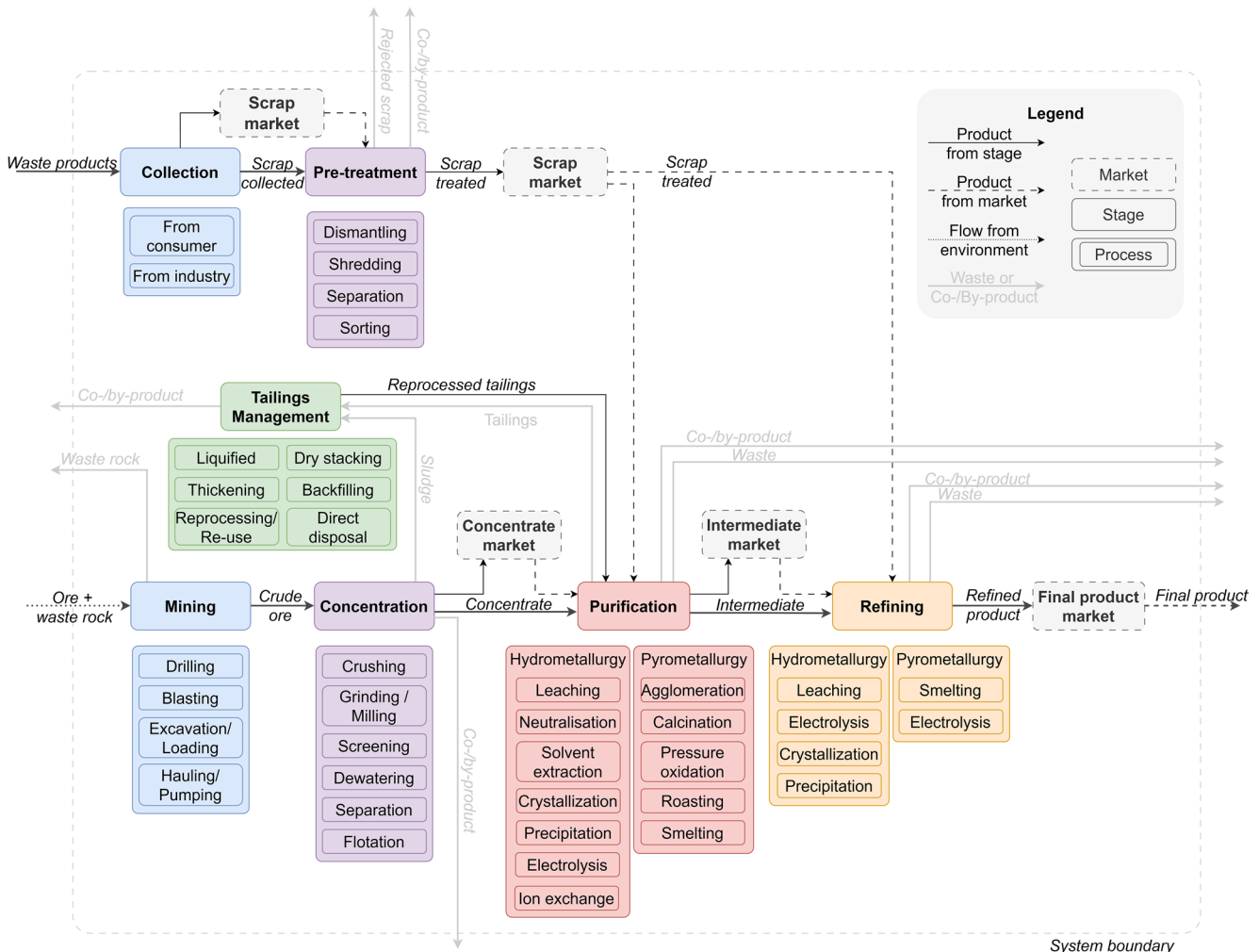
Fig. 2 Inventory model blueprint specifying life cycle stages, processes, and markets in the mineral value chain. Displayed in bold font are the life cycle stages, under them are their respective processes that can be used in the stage. Mining refers to the extraction of ore (e.g., nickel sulfide ore) and waste rock, concentration reduces ore size and increases the concentration of valuable material in the ore (e.g., milling and flotation of the sulfide ore), purification use hydro- or pyrometallurgical processes to further increase valuable material concentration (e.g., flash smelting to nickel matte), and refining produces the final product for further use in other applications (e.g., nickel class I production via Sherritt-Gordon process and further processing to nickel sulfate)
