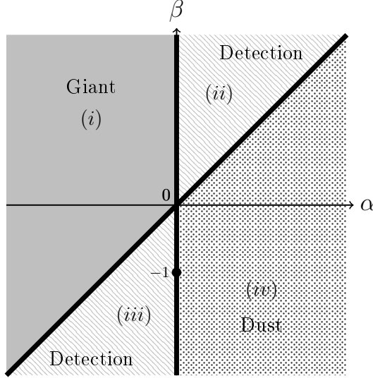
(b) Phase diagram for the community star graph, with q = n^\alpha and w = n^\beta . For each of the regions the following event occurs with high probability: (i) One single tree; (ii) k+1 trees, all k vertices incident to a weight 1 edge are isolated, while the remaining vertices form a single tree; (iii) n-k trees, all n-k-1 vertices incident to a weight w edge are isolated, while the remaining vertices form a single tree; (iv) n isolated vertices. The exact limit values of the correlations along the bold lines, i.e. in the non-degenerate regimes, can be found in Theorem 2.11.
