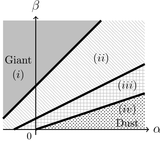
(b) Phase diagram for the complete d -ary hierarchical tree of height h = 3 , with d = n , q = n^\alpha and j -th generation edge weights w_j = n^{j\beta} for \beta \geq 0 . For each of the regions the following event occurs with high probability: (i) One single tree; (ii) All 2nd and 3rd generation edges are present, while all 1st generation edges are absent; (iii) All 3rd generation edges are present, while all 1st and 2nd generation edges are absent; (iv) All 1 + n + n^2 + n^3 vertices are isolated.
