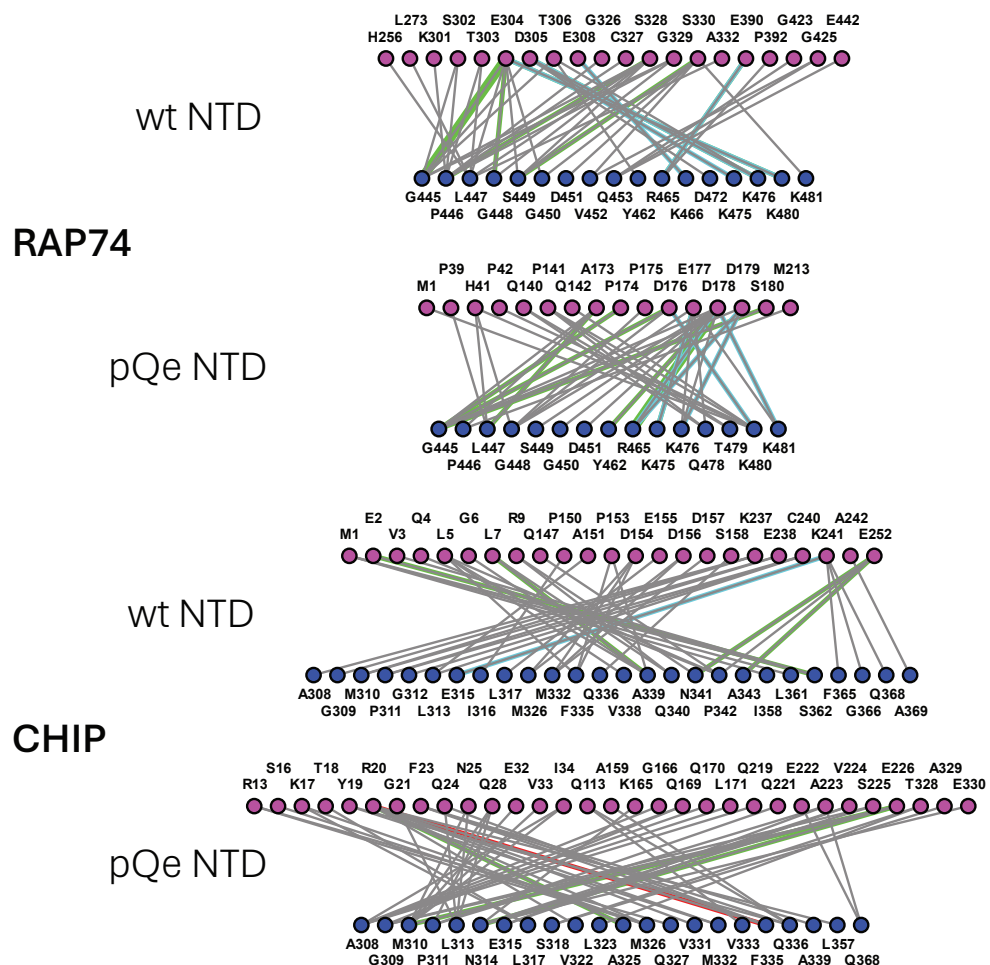
Figure S7. Interaction network of AR-NTD residues (top row, magenta spheres) with RAP74 and CHIP (bottom row, blue spheres). Different types of interactions are coloured differently: hydrogen bonds (green), salt-bridge/ionic (cyan), \pi -cation (red), and \pi -stacking (blue).
