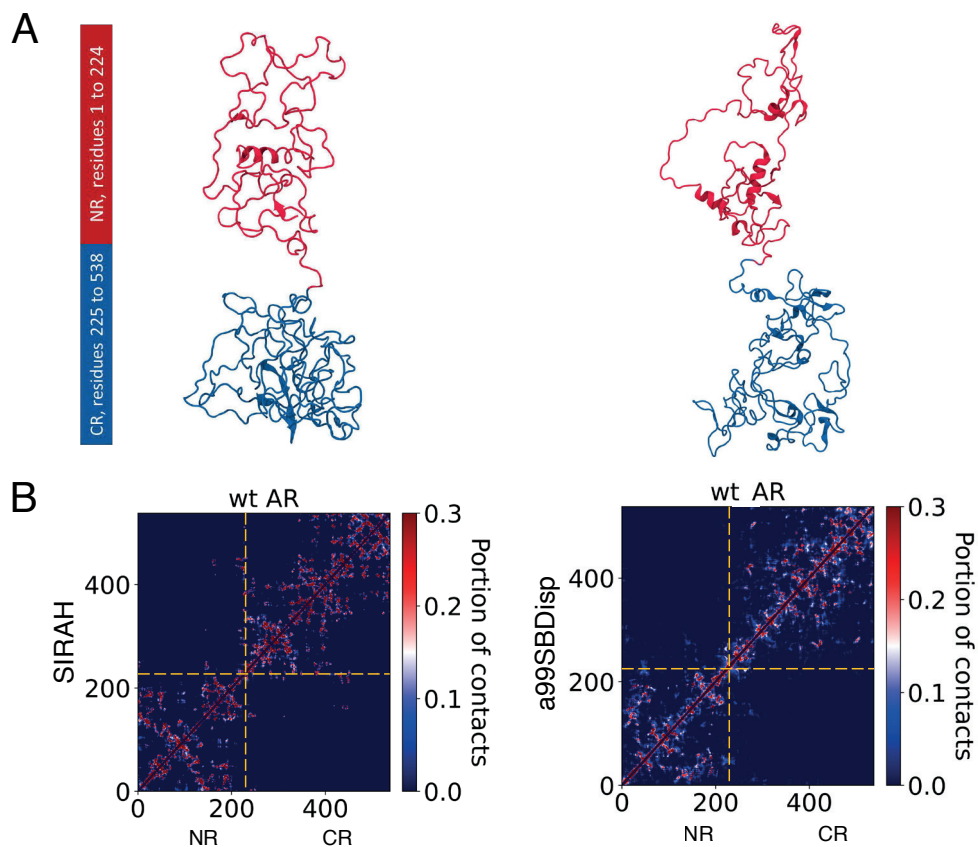
Figure S1. Regional segregation of wt-NTD. (A) NR and CR subregion segregation in NTD is obtained with both coarse-grained SIRAH (left) and all-atom a99SB-disp (right) forcefields. (B) Contact maps of the three all atom simulations combined highlights dynamic regional segregation of NTD into NR and CR as seen both in SIRAH and a99SB-disp generated models.
