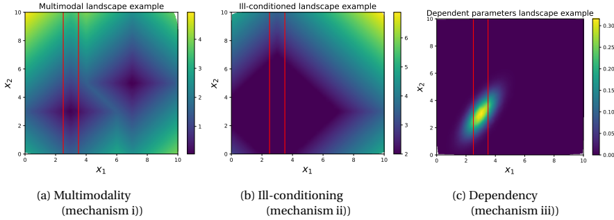
Figure 5.2: Examples of landscapes and the possible mechanisms of reduced ill-posedness through range constraint priors on the x_1 variable (red vertical lines). In Figure 5.2a, the constraint on the x_1 variable excludes the second optimum at (7, 5), thereby reducing ill-posedness through mechanism i). In Figure 5.2b, there are many points with a value very close to 2 (plotted simply as 2 for illustrative purposes), but the range constraint prevents errors larger than 1 (the width of the range) through mechanism ii); without the constraint, the model may have predicted points like (4, 6). Finally, in Figure 5.2c (where, for plotting convenience, we are maximising instead of minimising), due to the dependency between x_1 and x_2 , the range constraint prior on x_1 reduces the viable range for x_2 from about [1, 5] to about [1.5, 4.5] through mechanism iii).
