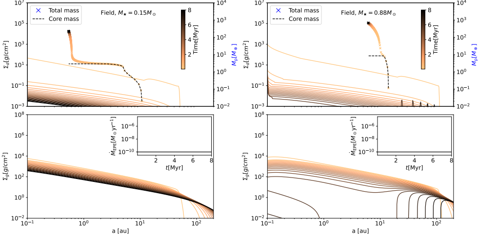
Figure 5.4. Comparison of disk evolution and planet growth tracks between a low-mass star ( 0.15M_\odot , left panels) and a relatively high-mass star ( 0.88M_\odot , right panels) in an isolated environment ( \dot{M}_{\text{EPE}} = 10^{-10} M_\odot \text{yr}^{-1} ). In the top panels, we display the evolution of dust surface density (left axis) alongside planet mass (right axis). The planet’s total mass and core mass are tracked separately using cross dots and dashed lines, respectively. The bottom panels show the evolution of gas surface density. The inset in the top right corner illustrates the history of external photo-evaporation rates experienced by the system. Both the top and bottom panels in each column share the same color bar, indicating the age of the system.
