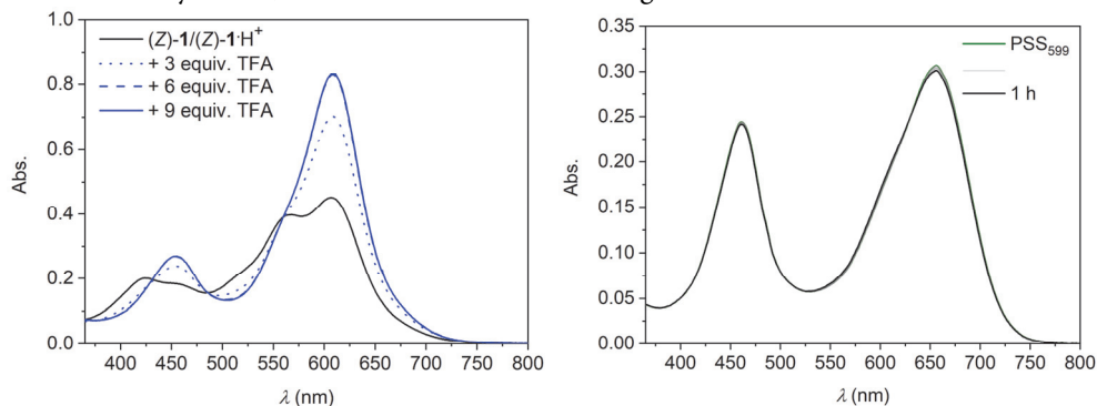
Figure E1. (left) UV-Vis spectral changes of a solution of as-isolated (Z)-1-TFA (15 \mu M in MeOH) upon addition of more TFA (0.05 M in MeOH). (right) UV-Vis spectra of ( E PSS )-1-H + (10 \mu M in MeOH, 12 equiv. of TFA) in the dark (600 s interval); DAbs. (at 655 nm) \leq 2% after 1 h, highlighting the thermal stability.
