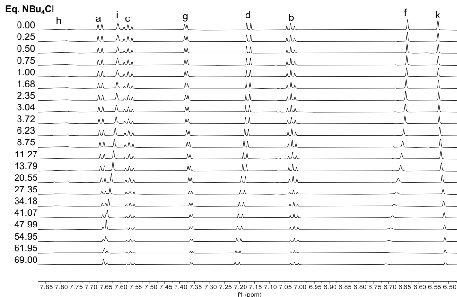
Figure E7. 1 H NMR spectra (600 MHz, MeOD) of ( Z )- 1 -H + (1 mM, 2 equiv. TFA) upon incremental addition of NBu 4 Cl (100 mM and 1.0 M).
