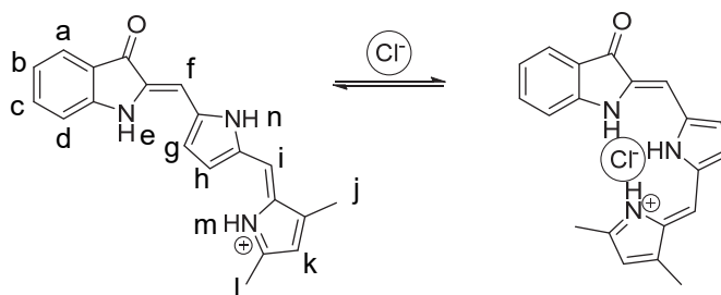
Scheme E1. Scheme of binding equilibrium including the lettering assignment of (Z)\text{-}1\text{-H}^+ .
