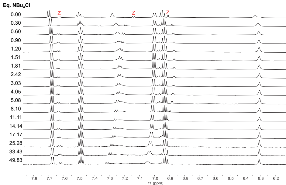
Figure E6. 1 H NMR spectra (600 MHz, CD 2 Cl 2 /MeOD 95:5 v/v) of ( E PSS )- 1 -H + (1 mM, 4 equiv. of TFA) upon incremental addition of NBu 4 Cl (100 mM). By relative 1 H NMR signal integration, an E / Z ratio of 16:84 was determined at the start of the titration.
