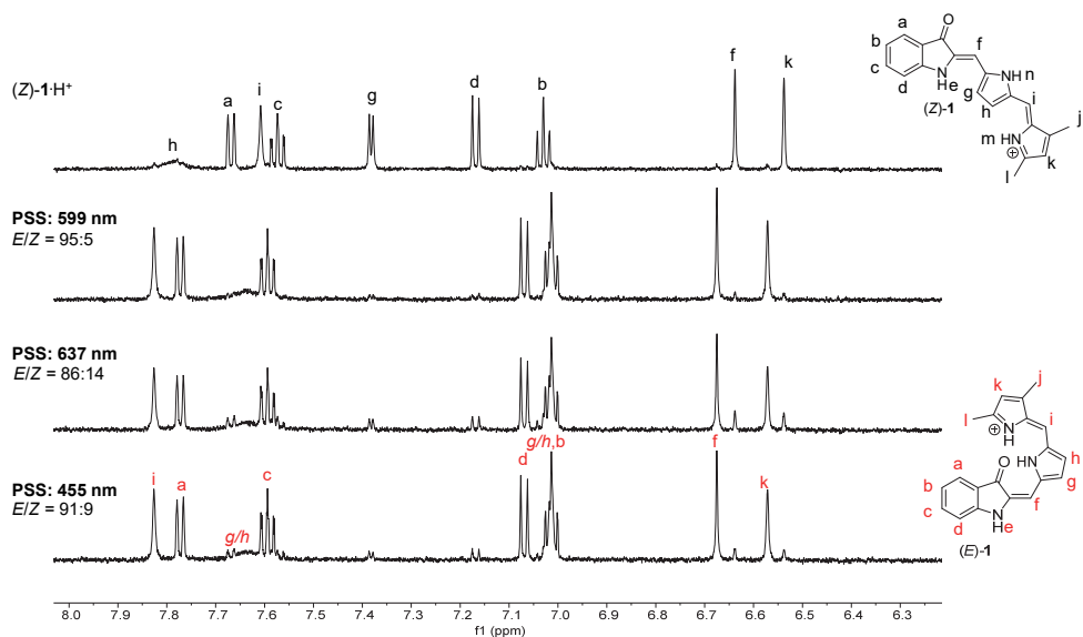
Figure E4. Aromatic region in the ^1\text{H} NMR spectra (600 MHz, MeOD) of (Z)-1-H + (0.15 mM, 10 equiv. TFA) upon sequential irradiation with 599 nm, 637 nm and 455 nm light. The integrals of signals Hl and Hj were used to calculate the PSS ratios.
