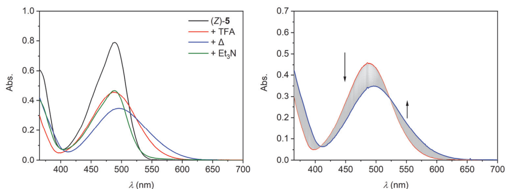
Figure E23. (left) UV-Vis spectra data of 5 (0.71 mM in degassed CHCl 3 , 1 mm quartz cuvette) before and after addition of excess TFA ( 3.7 \times 10^2 equiv.) [(Z)- 5H + ], followed by equilibration for 16 h [Δ, enriched in (E)- 5H + ], and treatment with Et 3 N (4.2 equiv. with respect to TFA) [enriched in (E)- 5 ]. (right) UV-Vis spectra data of 5 (0.71 mM in degassed CHCl 3 , 1 mm quartz cuvette) before and after addition of excess TFA ( 3.7 \times 10^2 equiv.) [(Z)- 5H + ], followed by equilibration for 16 h [Δ, enriched in (E)- 5H + ], and treatment with Et 3 N (4.2 equiv. with respect to TFA) [enriched in (E)- 5 ].
