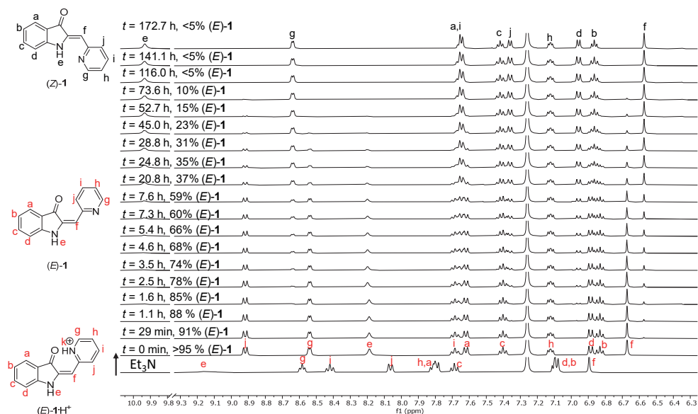
Figure E6. ^1\text{H} NMR spectral changes (400 and 500 MHz, \text{CDCl}_3 ) of ( E )-1· \text{H}^+ (5.7 mM) equilibrated in the presence of 32 equiv. of TFA followed over time (from bottom to top) after addition of 48 equiv. of \text{Et}_3\text{N} . The isomer ratio was determined by integration of the alkene Hf signals. Minor precipitation was observed during overnight measurements (between t = 7.6 h and 20.8 h) and sonication was therefore applied to the sample to ensure homogeneity. Note that upon addition of base most pyridyl proton signals shift upfield, indicative of deprotonation. The signal of pyridyl proton Hj, however, was found to shift downfield. Upon deprotonation, the pyridyl nitrogen will likely rotate away from the carbonyl group, placing this pyridyl proton in close proximity to the anisotropic carbonyl deshielding cone.
