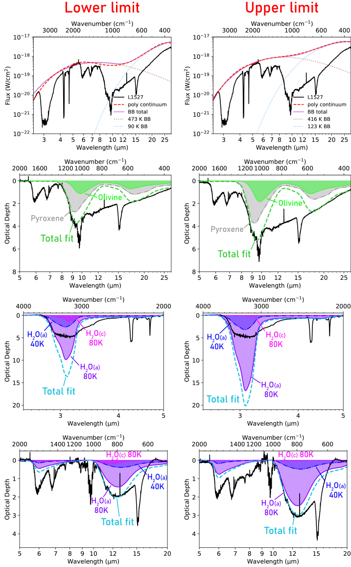
Figure 3.A.12: The global continua and subsequent silicate subtractions and H 2 O ice fits used to define continuum uncertainties on the H 2 O column densities. First row: the lower (left) and upper (right) limits on the global continua in the central spectrum. Second row: the silicate subtraction performed on the optical depth-scale spectra extracted using the continua in the top row. Third and fourth row: H 2 O ice fits to the NIRSpc and silicate-subtracted MIRI spectra. The resulting H 2 O column densities were used to define the H 2 O column density uncertainty from the continuum choice.
