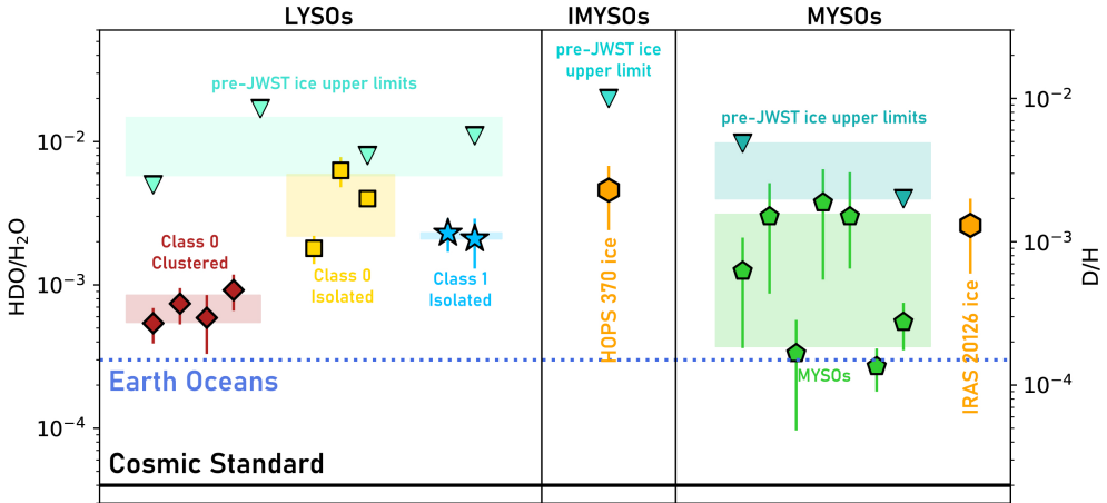
Figure 2.8: Comparison of HDO/H 2 O ratios measured in the gas and ice toward protostars of various masses (adapted from Jensen et al. 2019 and Andreu et al. 2023). Ratios measured in the gas phase are plotted with red diamonds for clustered Class 0 LYSOs, yellow squares for isolated Class 0 LYSOs, blue stars for isolated Class 1 LYSOs, and green pentagons for MYSOs. Ice upper limits derived from pre-JWST spectra are plotted with teal triangles. The JWST ice values from this work are plotted with orange hexagons. The literature values used in this figure are provided in Table 2.A.10.
