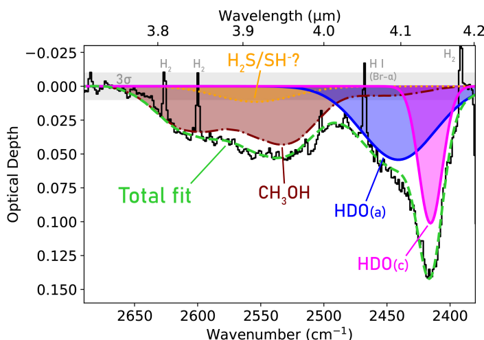
Figure 3.2: NIRSpect spectrum of L1527 on the optical depth scale from 3.7–4.2 \mu\text{m} (solid black trace) along with the ice fit components \text{CH}_3\text{OH} (dash-dotted brown trace), a Gaussian representing \text{SH} -bearing ices (dotted yellow trace), amorphous HDO (solid blue trace), crystalline HDO (solid magenta trace), and the total combined ice fit (dashed green trace). The gray horizontal shaded region indicates the 3\sigma noise level. See Figure 3.A.5 for the local continuum used to extract this spectrum.
