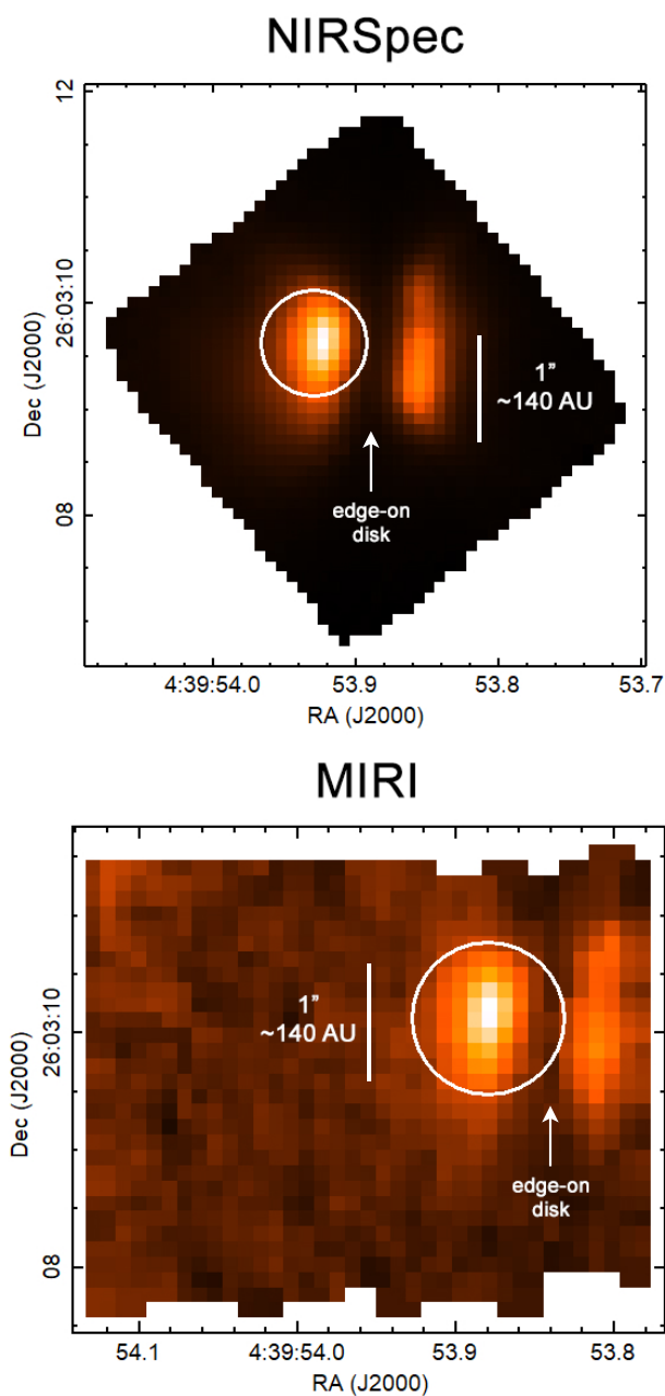
Figure 3.1: 5 \mu\text{m} continuum maps from the L1527 datacubes collected via NIRSpec IFU G395M (top) and MIRI-MRS (bottom) with the positions of the respective 1'' and 1.30'' diameter apertures used to extract the analyzed spectra shown in white.
