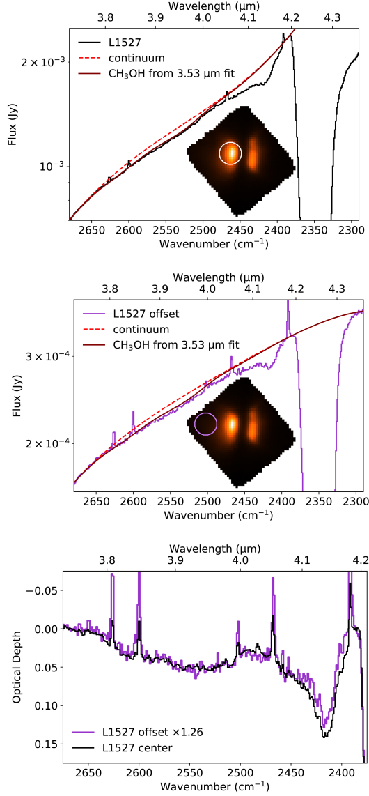
Figure 3.A.5: NIRSpec spectra of L1527 from 3.7-4.2 \mu\text{m} extracted with 1'' apertures from the region where the flux at 5 \mu\text{m} is maximized (top panel, black trace) and the region where ice absorption features are still present, but the CO 2 scattering wing is minimized (middle panel, purple trace). The dashed red traces indicate the local continua fit to these spectral regions, and the insets show the respective extracted regions in the NIRSpec datacube. The bottom panel compares the extracted optical depth spectra resulting from these local continuum fits to the two spectra. The local continuum in the top panel was used to calculate the optical depth spectrum presented in Figure 3.2.
