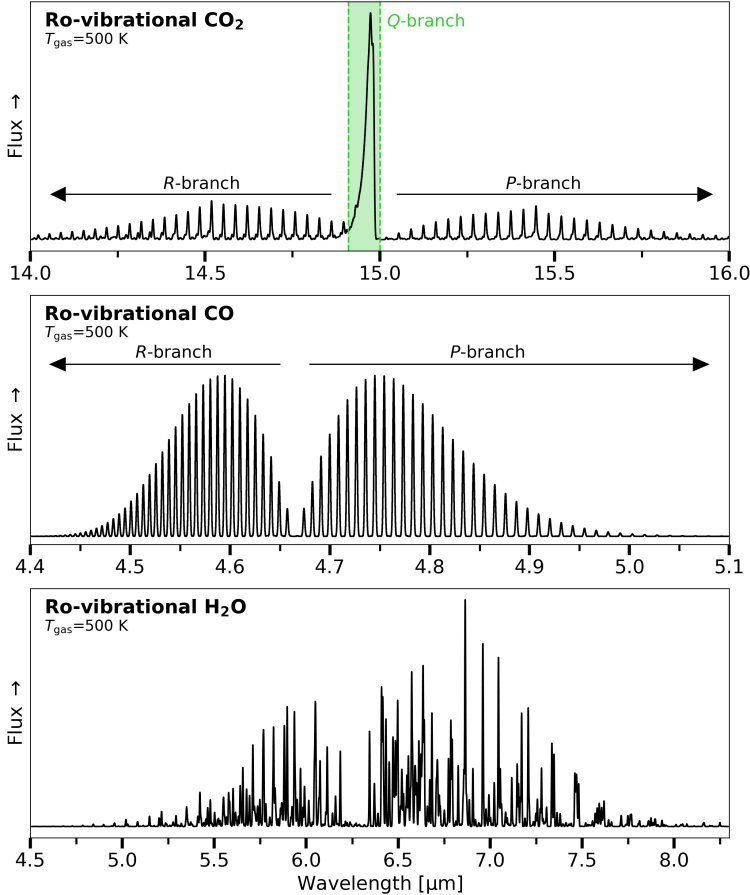
Figure 1.12: Simulated, optically thin ro-vibrational spectra of \text{CO}_2 (top panel), \text{CO} (middle panel), and \text{H}_2\text{O} (bottom panel) at T_{\text{gas}} = 500 K. The Q -, P - and R -branches of \text{CO}_2 and the P - and R -branches of \text{CO} are indicated.
