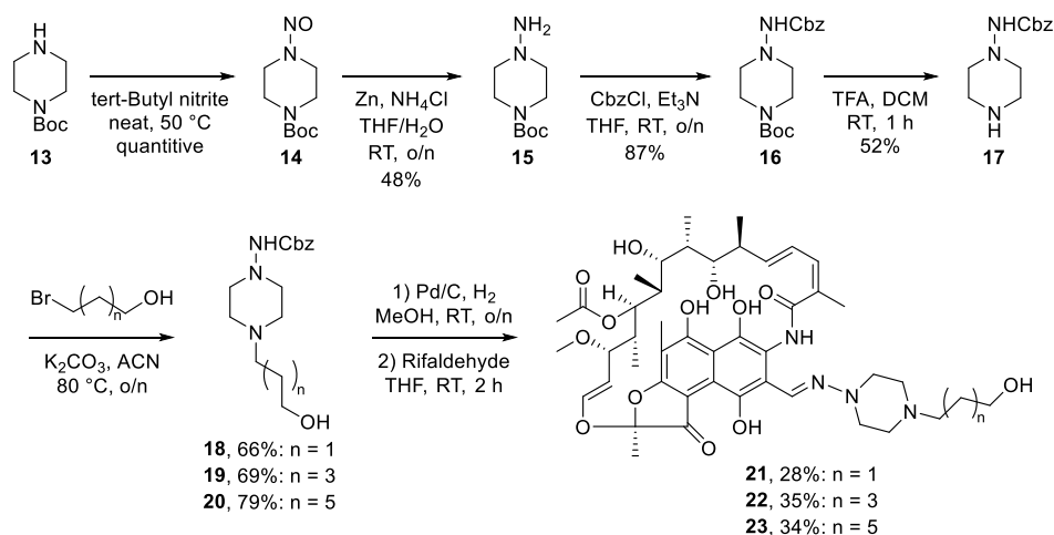
Scheme 2. Synthesis of the rifampicins modified with different alcohol-containing linkers.
