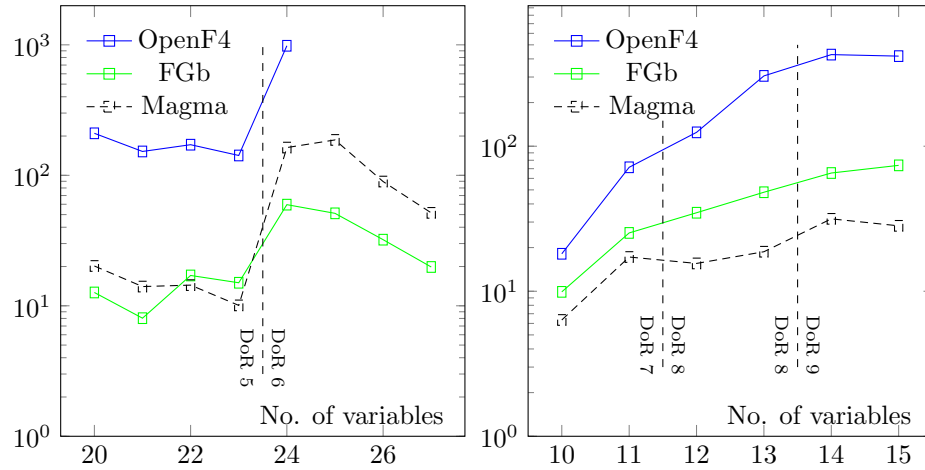
Figure 3: The ratio of time-memory product of Magma, FGb, and OpenF4 relative to the time-memory product of M4GB. The left graph is the result on systems with n variables and 2n equations whereas the right one is the result on systems with n variables and n + 1 equations. The vertical dashed line separates the parameter with different degree of regularity (DoR).
