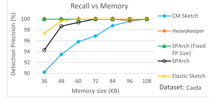
Fig. 18. Flow detection: recall vs memory size.
