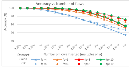
Fig. 19. Accuracy vs number of flows (SPArch).
