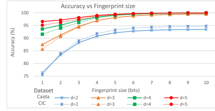
Fig. 20. Accuracy vs Fingerprint size (SPArch).
