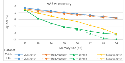
Fig. 12. AAE vs memory size.
