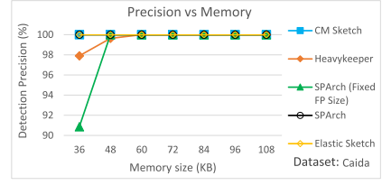
Fig. 16. Flow detection: precision vs memory size.
