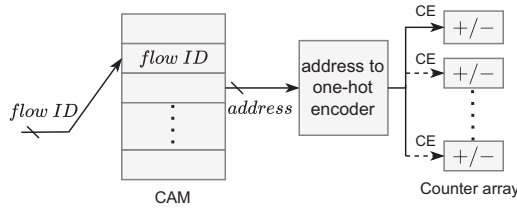
Fig. 1. CAM-based counter array.
