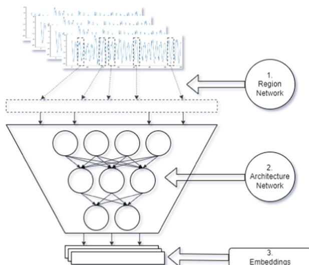
Fig. 3 Graphical overview of AutoPOI framework
