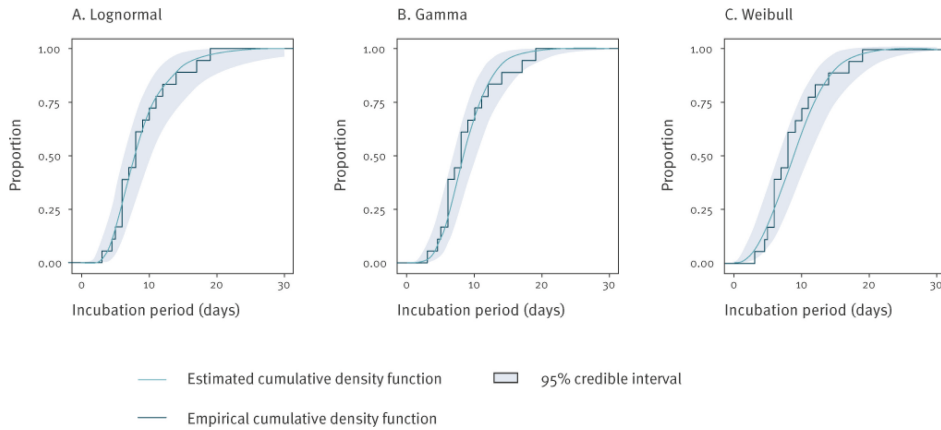
Figure. Estimated cumulative density functions, according to different parametric distributions and empirical cumulative density function of incubation periods reported for monkeypox cases in the Netherlands, May 2022 (N = 18 cases) For the visualisation of the empirical cumulative distribution, the median points of the reported time interval of exposure were used.
