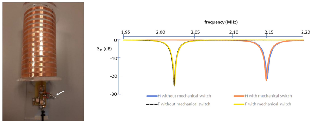
Fig. 1. (left) Photograph of the solenoid coil which can be switched between ^1\text{H} and ^{19}\text{F} using a mechanical switch (arrow). (right) S_{11} plots of the ^1\text{H} and ^{19}\text{F} switched-mode RF coil. A comparison with/without the low-loss mechanical switch shows negligible differences.
