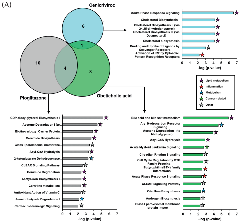
Figure 4. Early changes in hepatic transcriptomics profile in Ldlr -/- .Leiden mice on HFD treated with cenicriviroc, pioglitazone or obeticholic acid. Venn diagram (A) showing the overlap of differentially expressed pathways (DEPs) in the liver. Diet-induced obese mice received 4 weeks of high fat diet (HFD) feeding supplemented with cenicriviroc (blue circle), pioglitazone (gray circle) or obeticholic acid (green circle). DEPs per intervention are specified in (A). A gene signature of Ldlr -/- .Leiden mice that received 19 weeks of HFD feeding was used, in which 232 genes are described that predict MASH-associated fibrosis 1 . Expression of the genes comprising this signature was evaluated and for each gene, expression changes of the HFD control group versus chow control group was set at 100%. Treatment groups were compared to HFD controls and shown as box and whisker plot with 2.5–97.5 percentile whiskers (B). A heatmap (C) showing 2log fold changes (2logFC) of the top genes upregulated in the HFD group versus chow control and 2logFC of the same genes in treatment groups. Red color indicates upregulation and blue color indicates downregulation. Ceni, cenicriviroc; OCA, obeticholic acid; pio, pioglitazone.
