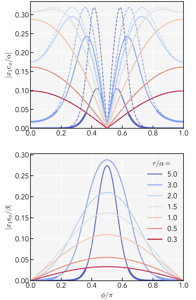
Figure 6. Similar to Fig. 5, we show the variation of the along-scan (top) and across-scan (bottom) position of the observed maxima, now in units of their relative width. Here we show the absolute value, noting that the actual sign of the observed offset is the same as the sign of the trigonometric term. In the across-scan plot, we also show (dashed lines) the offset as would be calculated taking \beta \rightarrow \infty .
