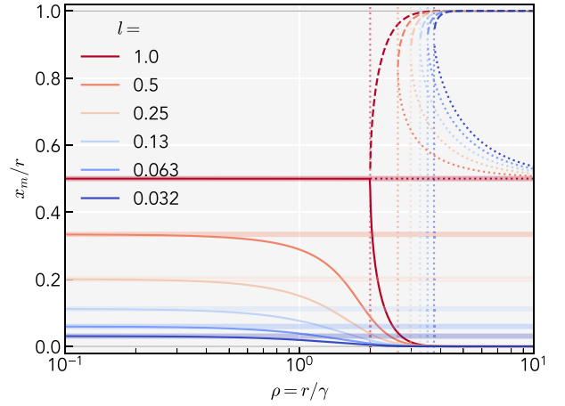
Figure 3. Here we show, as a function of \rho , the relative location of the primary maxima (solid line) and where present the secondary maximum (dashed line) and the minimum (dotted line), for various l . The dashed vertical lines show the critical \rho_c(l) above which a minimum exists. The wide translucent horizontal lines show x_m = x_0 , the asymptotic solution for the position of the primary maximum when \rho \ll 1 .
