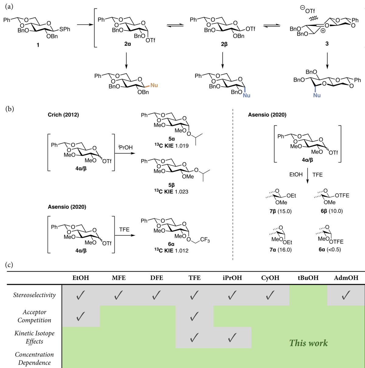
Fig. 1 (a) Mechanistic pathways to account for the selectivity in glycosylation reactions of the 4,6- O -benzylidene glucosyl donor, 1 . (b) Kinetic isotope effects (KIEs) for 1 i PrOH were recorded by Crich and coworkers on a similar, 2,3-di- O -methyl protected, glucosyl sulfoxide donor. 24 Acceptor competition experiments and KIE measurements for TFE were performed by Asensio and colleagues. 19 Numbers in brackets are relative formation rates for the O -glycosides in the competition experiments. (c) An overview of experiments performed in recent times to probe the mechanistic picture and the experiments that we present in this work.
