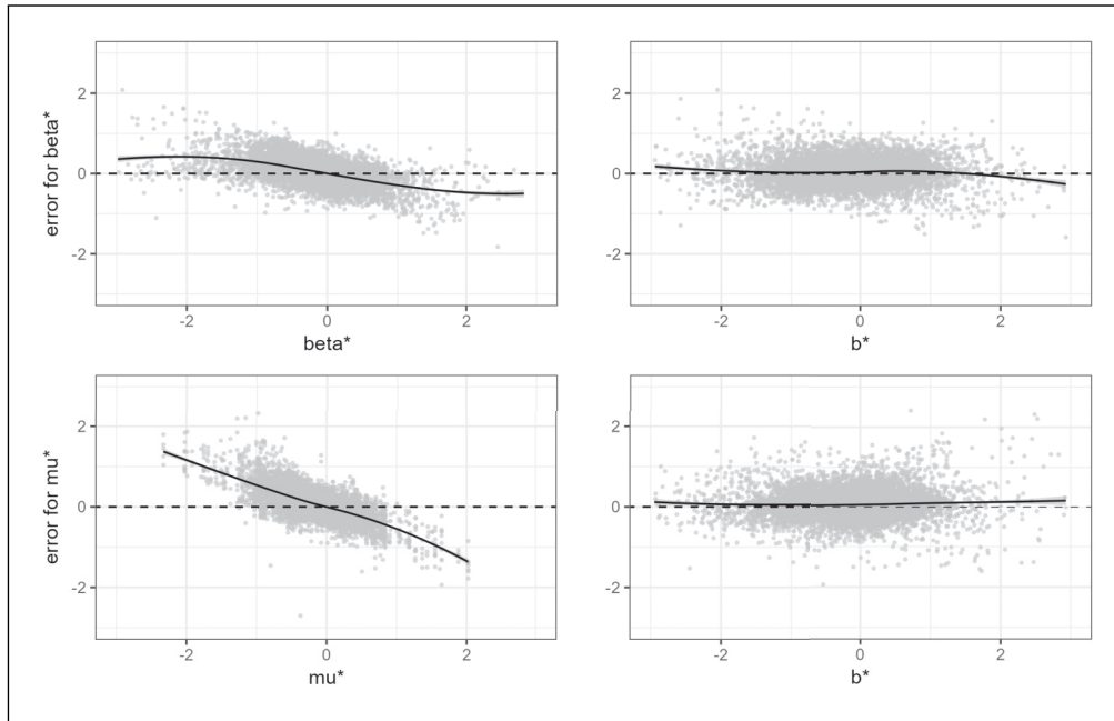
Figure 3. Bias of the proposed Bayesian estimators. The two top panels show \hat{\beta}_{ij}^* - \beta_{ij}^* . The two bottom panels show \hat{\mu}_{ij}^* - \mu_i^* . The two panels on the left side show the frequentist bias, while the two panels on the right side show the Bayesian bias.
