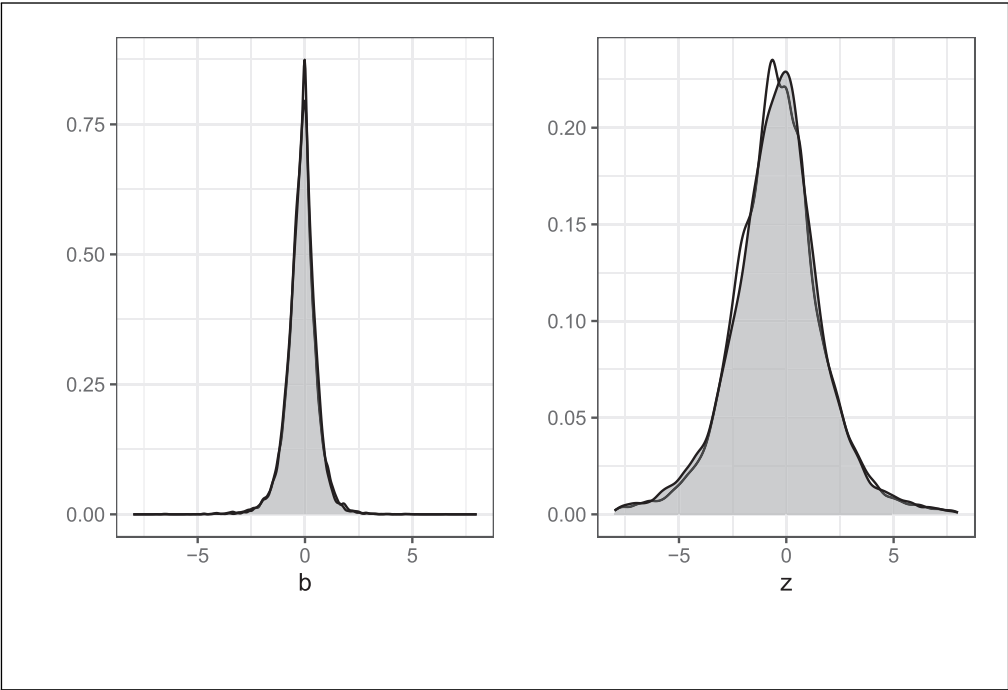
Figure 2. Observed and simulated distributions of 18,368 estimates and z-values.
