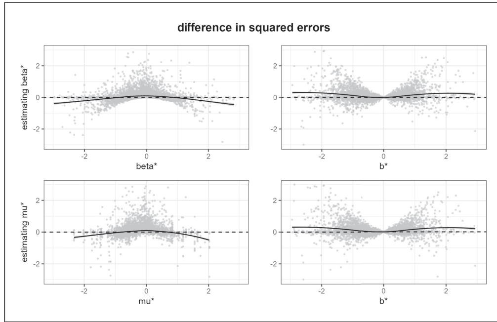
Figure 4. Difference in squared error of the naive and Bayesian estimators. Top row: difference in squared errors for \beta_{ij}^* from (8). Bottom row: difference in squared errors for \mu_i^* , from (9). The two panels on the left side show the frequentist perspective, while the two panels on the right side show the Bayesian perspective.
