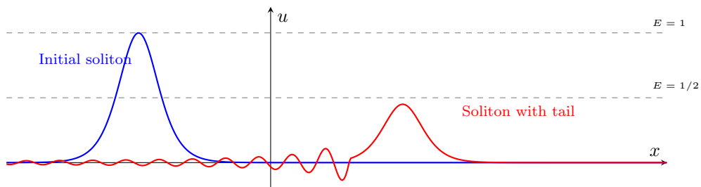
Figure 1.3: An initial solitary wave with energy 1 (blue) propagates through a dissipative medium, resulting in a total energy 1/2 . The resulting wave (red) has formed a dispersive tail, and has slightly less than half the original energy.
