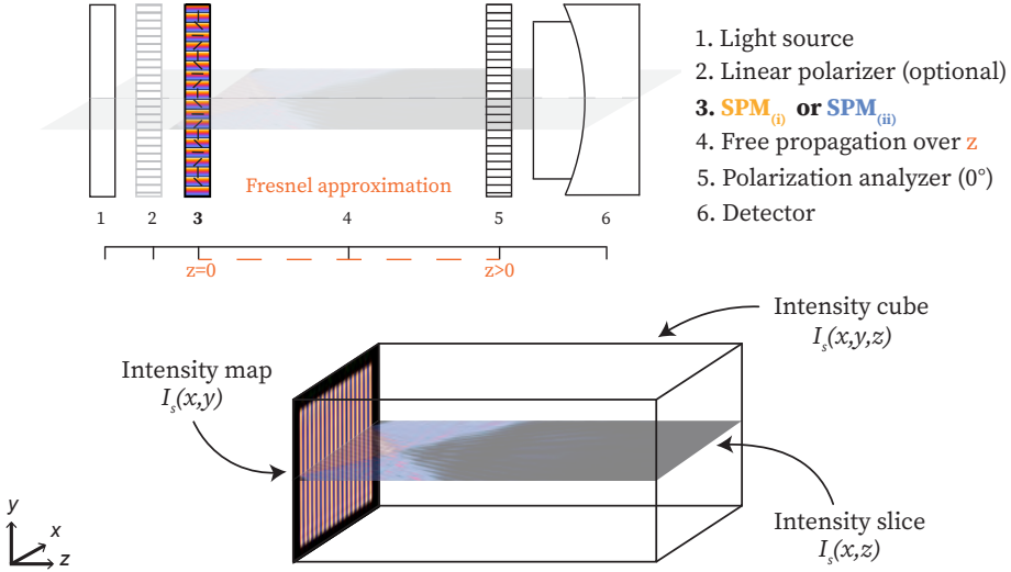
Figure 5.4: Top panel: A schematic overview of the simulated set-up. Bottom panel: Each simulation run returns an two-dimensional electric field x_i, y_i of a monochromatic propagated wavefront. An intensity cube I_s(x, y, z) is a stack of intensity maps I_s(x, y) , from which intensity slices, I_s(x, z) , can be retrieved.
