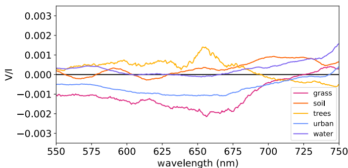
Figure 3.6: V/I spectra measured while pointing at various surfaces scenes : grass, soil, trees, urban, and (lake) water.
