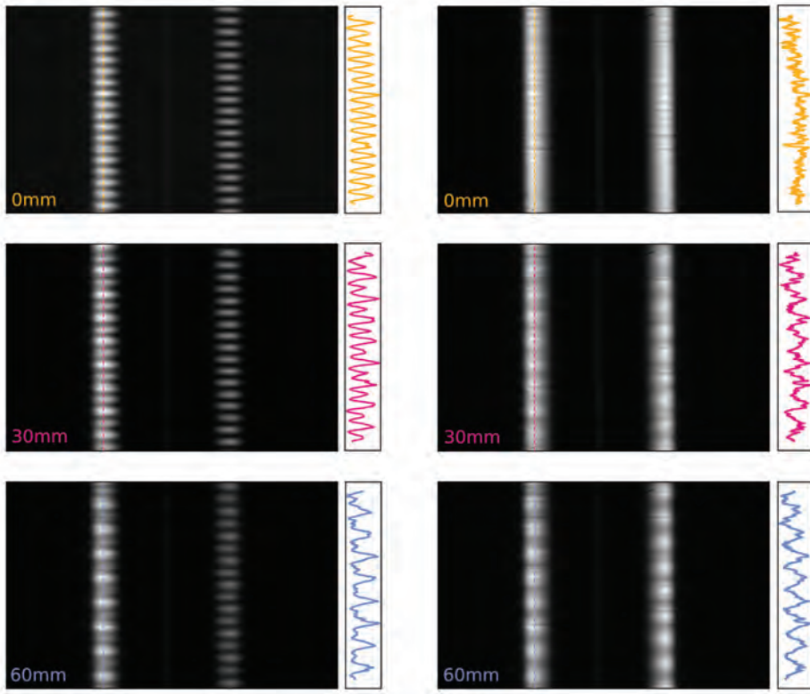
Figure 4.7: Detector images obtained with LSDPol using an light source that is linear polarised (Q, left panels ) and unpolarised ( right panels ). The polarisation modulator-slit distance was set to 1.5 \pm 2.0 mm (referred to as 0 mm), 31.5 \pm 2.0 mm (referred to as 30 mm) and 61.5 \pm 2.0 mm (referred to as 60 mm) ( top to bottom ). The coloured vertical lines mark the detector columns used to extract the intensity modulation shown beside each image.
