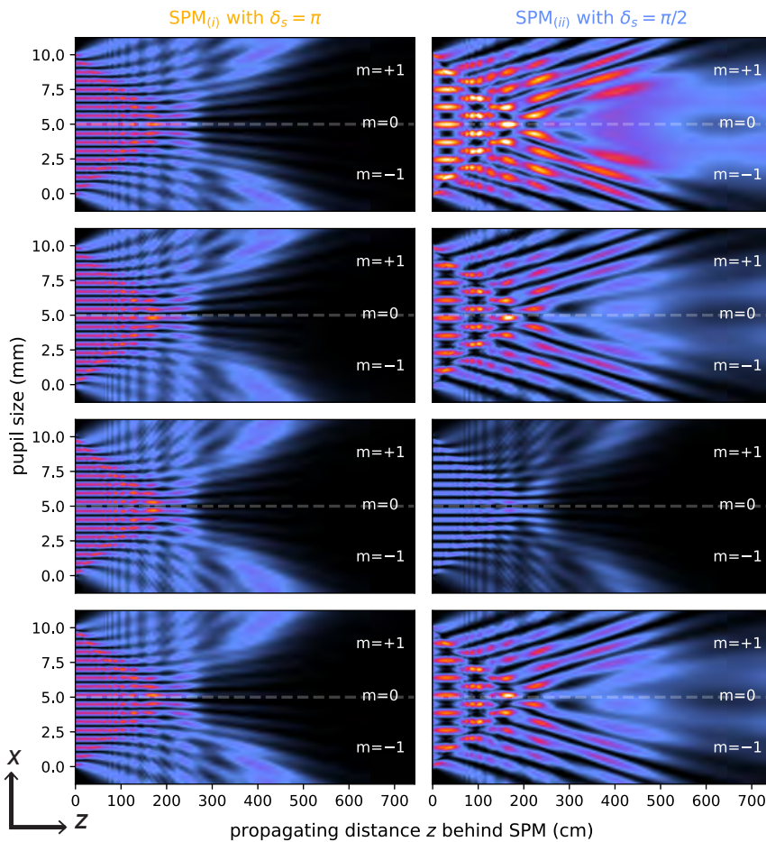
Figure 5.10: Intensity slices I_s(x, z) for z_{\max} \approx 7.5 m, depicting how incident linear polarised light emerges from SPM (i) SPM (ii) with a grating period of d = 0.3 mm and a wavelength of \lambda = 650 nm.
