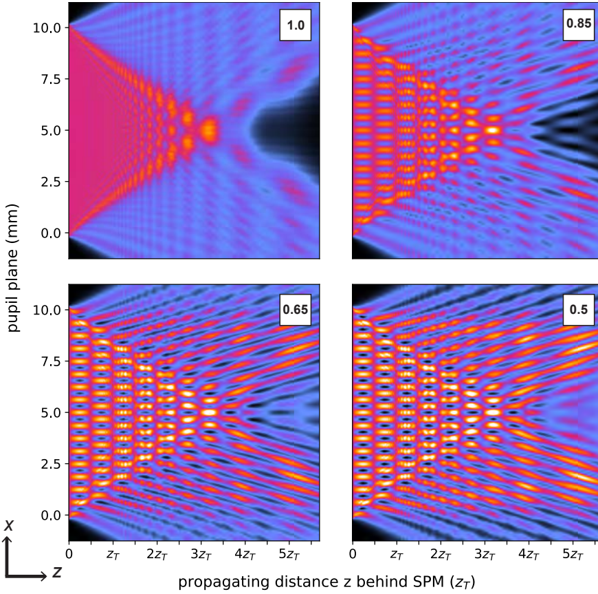
Figure 5.7: Intensity slices I_s(x, z) for z_{\max} \approx 3.5\text{m} \sim 5.8z_T , z_{\max} = 3.5\text{ m} and \Delta z = 0.007\text{ m} , depicting how incident unpolarised light ( \lambda = 550\text{ nm} ) emerges from \text{SPM}_{(\text{iii})} , with a grating period of d = 0.3\text{ mm} , and a linear polariser behind the SPM. From top left to bottom right, the retardance varies from half-wave ( \eta_{\text{pl}} = 1.0 ) to quarter-wave ( \eta_{\text{pl}} = 0.5 ).
