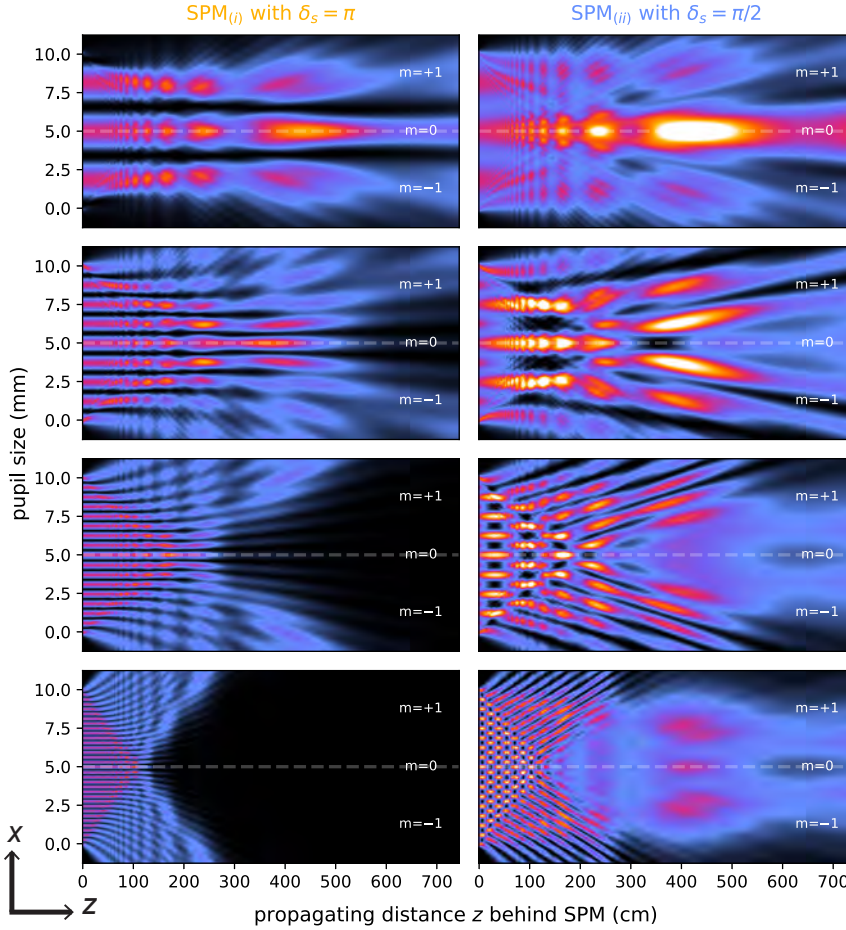
Figure 5.9: Intensity slices I_s(x, z) for z_{\max} \approx 7.5 m, depicting how incident unpolarised light with a wavelength of \lambda = 650 nm emerges from \text{SPM}_{(i)} and \text{SPM}_{(ii)} with a varying grating period d of 1.2, 0.6, 0.3, and 0.15 mm (from top to bottom).
