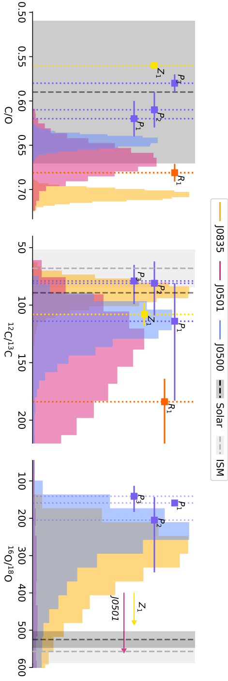
Figure 2.4: Posterior distributions of the C/O (left), carbon ^{12}\text{C}/^{13}\text{C} isotope (middle), and oxygen ^{16}\text{O}/^{18}\text{O} isotope ratio (right) for J0835, J0501 and J0500. The ^{12}\text{C}/^{13}\text{C} values for the Solar System (terrestrial value) and ISM are 89.3 \pm 0.2 (Meija et al., 2016) and 68 \pm 16 (Milam et al., 2005), respectively. The C/O value for our Sun is 0.59 \pm 0.08 (Asplund et al., 2021). The ^{16}\text{O}/^{18}\text{O} values for the Solar System and ISM are 557 \pm 30 (Wilson, 1999) and 525 \pm 21 (Lyons et al., 2018). The purple error bars represent the young BDs observed and analysed by González Picos et al. (2024, P 1 : J1200, P 2 : TWA28 and P 3 : J0856), the orange error bar DENIS J0255 (R 1 ) by de Regt et al. (2024), and the yellow 2M0355 (Z 1 ) by Zhang et al. (2022).
