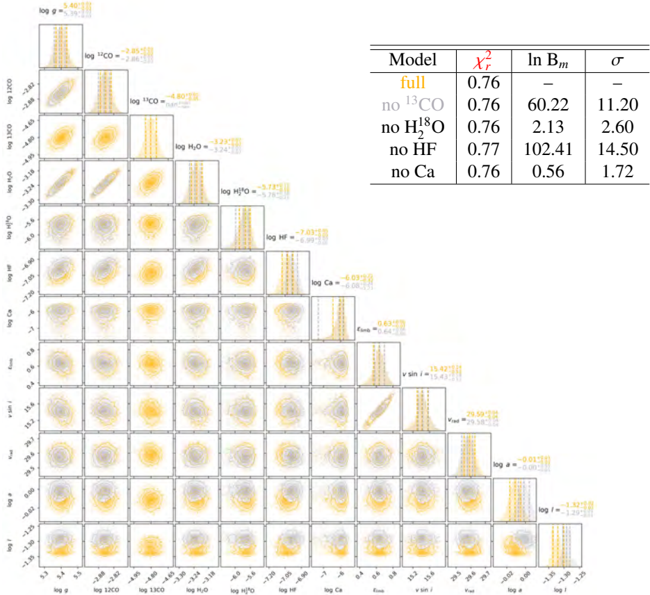
Figure 2.8: Posterior distributions of the retrieved parameters for J0835 . In yellow, we show the distributions for a model fitted for 21 free parameters including ^{12}\text{CO} , ^{13}\text{CO} , \text{H}_2^{16}\text{O} , \text{H}_2^{18}\text{O} , HF and Ca. The grey distributions represent a model where ^{13}\text{CO} is excluded. The reduced chi-squared values for the models with and without ^{13}\text{CO} , \text{H}_2^{18}\text{O} , HF and Ca are shown in the top right corner.
