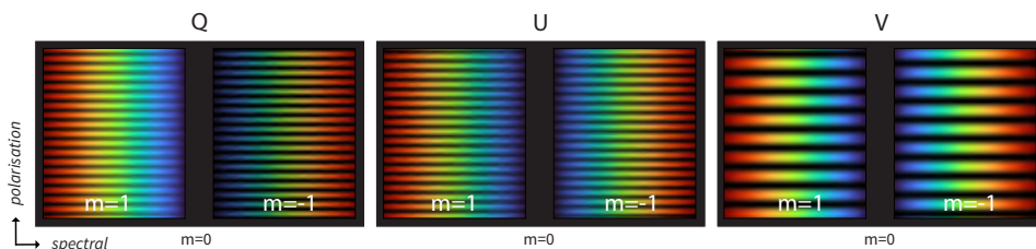
Figure 4.2: Left to right: Simulated intensity I' (detector images) resulting from fully polarised incident light \pm Q, \pm U, \pm V . The vertical polarisation dimension reveals the sinusoidal observed intensity modulation. The fake colours indicate how the light spectrum would be distributed over the horizontal spectral axis of the detector and the brightness shows the intensity modulation. Note these images are created using trivial calculations of an observed intensity from Mueller matrix calculations.
